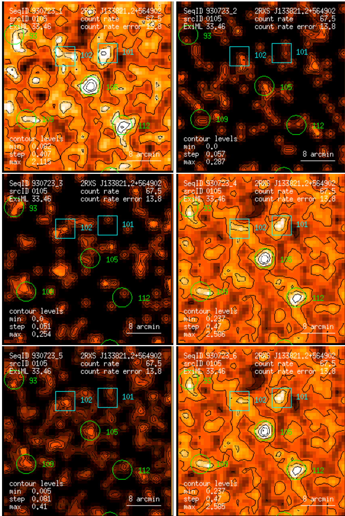
Figure 105: RASS 930723: detection 0105: band rate images, Gaussian filter: (1) PSPC channels 11 – 41, (2) 52 – 90, (3) 91 – 201, (4) 11 – 235, (5) 52 – 201, (6) 11 – 201. Broad band rates in counts/ks. Band rate contour levels in counts/ks/arcmin 2 .
