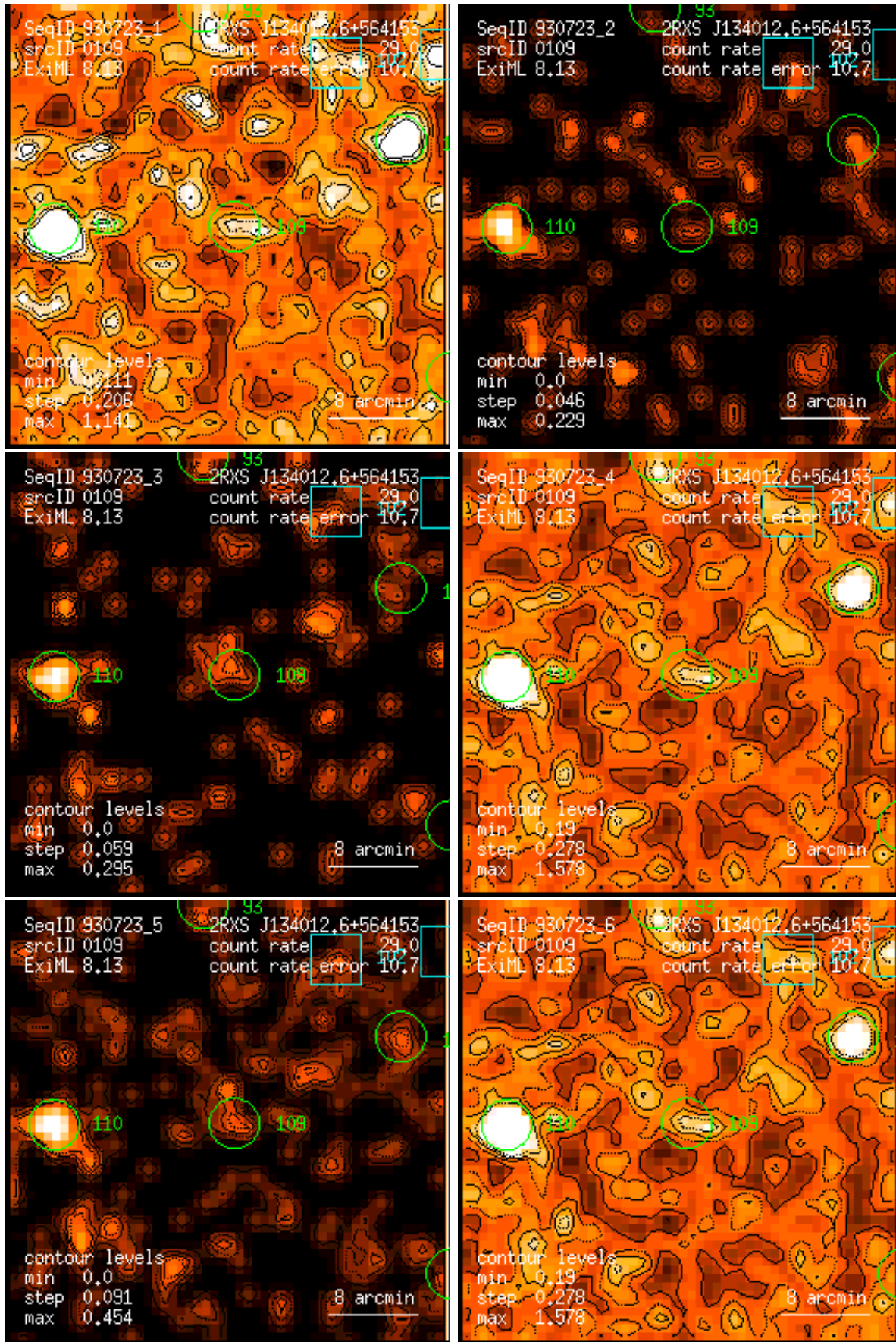
Figure 109: RASS 930723: detection 0109: band rate images, Gaussian filter: (1) PSPC channels 11 – 41, (2) 52 – 90, (3) 91 – 201, (4) 11 – 235, (5) 52 – 201, (6) 11 – 201. Broad band rates in counts/ks. Band rate contour levels in counts/ks/arcmin 2 .
