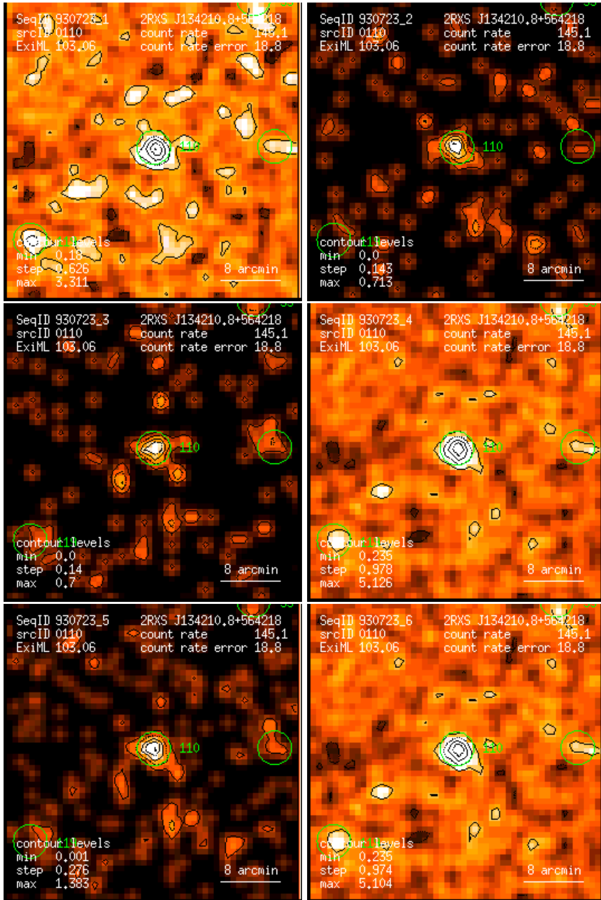
Figure 110: RASS 930723: detection 0110: band rate images, Gaussian filter: (1) PSPC channels 11 – 41, (2) 52 – 90, (3) 91 – 201, (4) 11 – 235, (5) 52 – 201, (6) 11 – 201. Broad band rates in counts/ks. Band rate contour levels in counts/ks/arcmin 2 .
