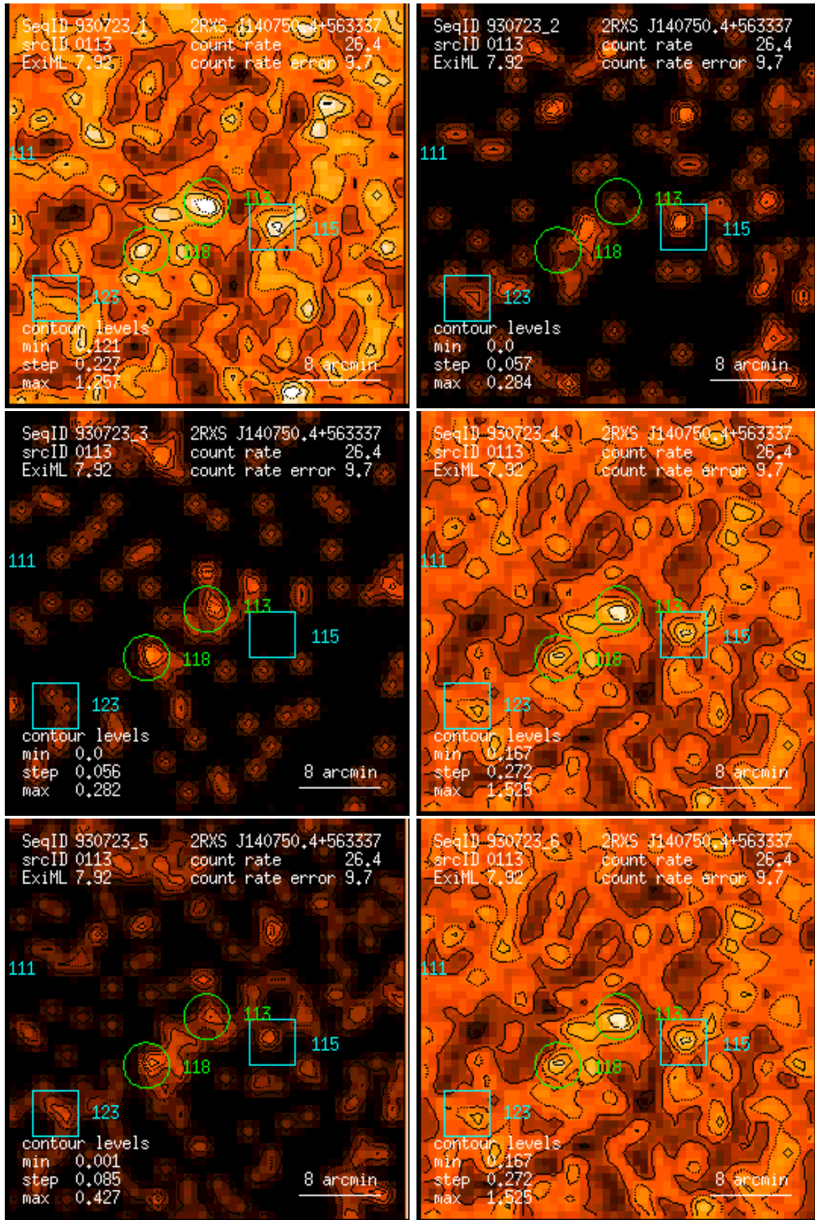
Figure 113: RASS 930723: detection 0113: band rate images, Gaussian filter: (1) PSPC channels 11 – 41, (2) 52 – 90, (3) 91 – 201, (4) 11 – 235, (5) 52 – 201, (6) 11 – 201. Broad band rates in counts/ks. Band rate contour levels in counts/ks/arcmin 2 .
