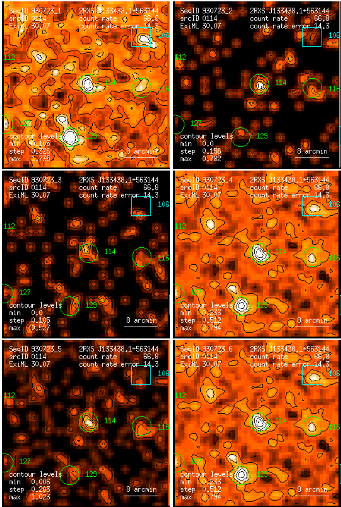
Figure 114: RASS 930723: detection 0114: band rate images, Gaussian filter: (1) PSPC channels 11 – 41, (2) 52 – 90, (3) 91 – 201, (4) 11 – 235, (5) 52 – 201, (6) 11 – 201. Broad band rates in counts/ks. Band rate contour levels in counts/ks/arcmin 2 .
