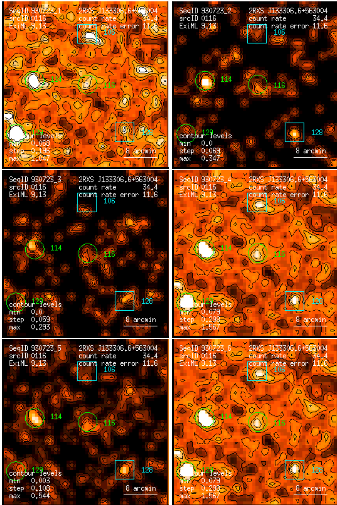
Figure 116: RASS 930723: detection 0116: band rate images, Gaussian filter: (1) PSPC channels 11 – 41, (2) 52 – 90, (3) 91 – 201, (4) 11 – 235, (5) 52 – 201, (6) 11 – 201. Broad band rates in counts/ks. Band rate contour levels in counts/ks/arcmin 2 .
