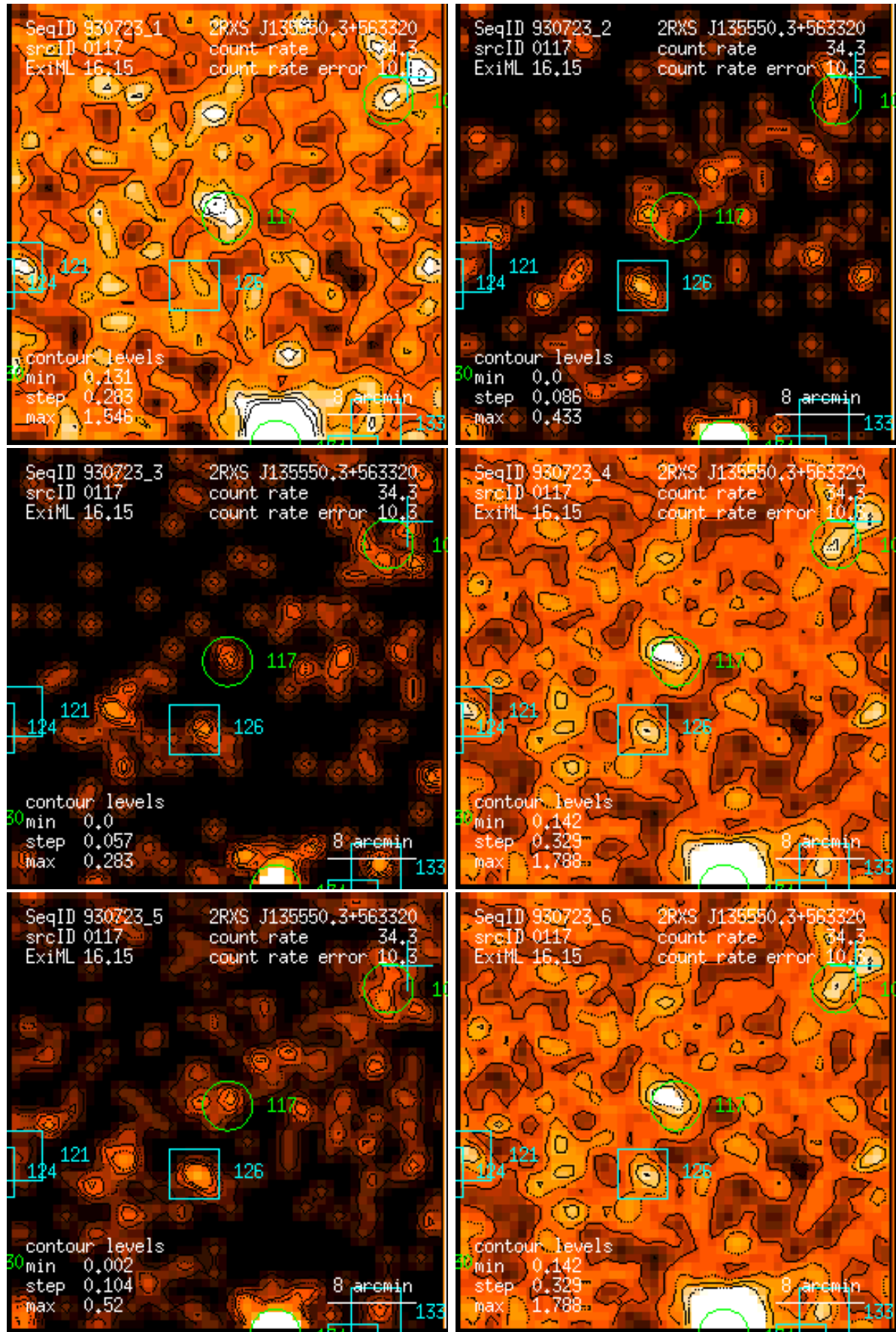
Figure 117: RASS 930723: detection 0117: band rate images, Gaussian filter: (1) PSPC channels 11 – 41, (2) 52 – 90, (3) 91 – 201, (4) 11 – 235, (5) 52 – 201, (6) 11 – 201. Broad band rates in counts/ks. Band rate contour levels in counts/ks/arcmin 2 .
