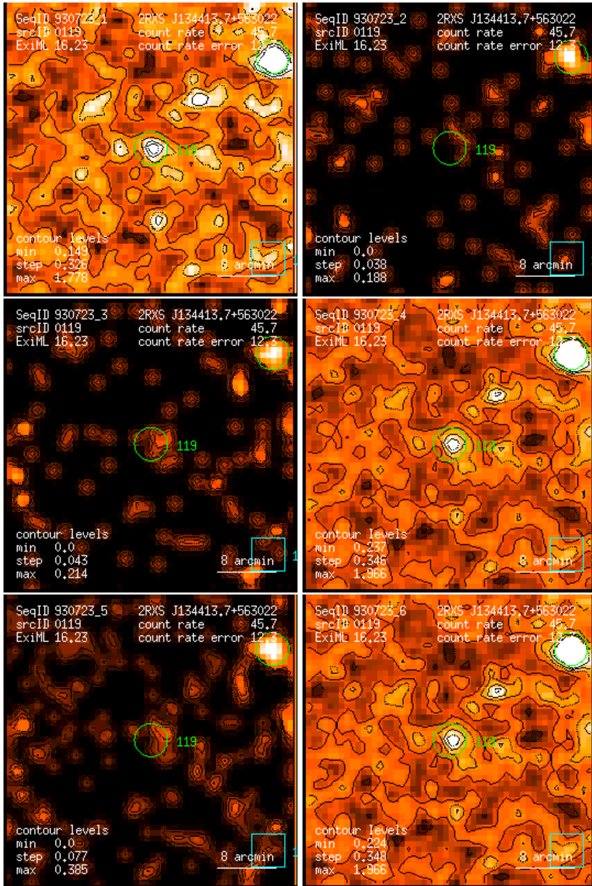
Figure 119: RASS 930723: detection 0119: band rate images, Gaussian filter: (1) PSPC channels 11 – 41, (2) 52 – 90, (3) 91 – 201, (4) 11 – 235, (5) 52 – 201, (6) 11 – 201. Broad band rates in counts/ks. Band rate contour levels in counts/ks/arcmin 2 .
