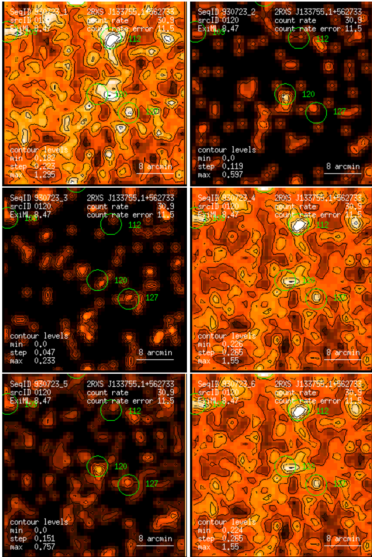
Figure 120: RASS 930723: detection 0120: band rate images, Gaussian filter: (1) PSPC channels 11 – 41, (2) 52 – 90, (3) 91 – 201, (4) 11 – 235, (5) 52 – 201, (6) 11 – 201. Broad band rates in counts/ks. Band rate contour levels in counts/ks/arcmin 2 .
