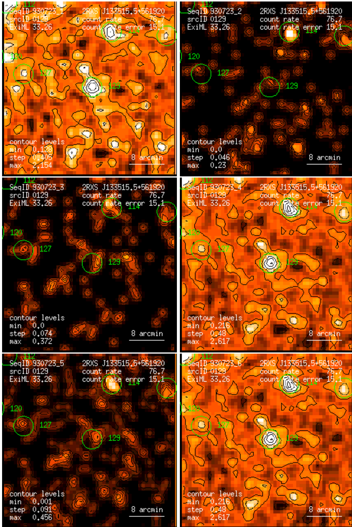
Figure 129: RASS 930723: detection 0129: band rate images, Gaussian filter: (1) PSPC channels 11 – 41, (2) 52 – 90, (3) 91 – 201, (4) 11 – 235, (5) 52 – 201, (6) 11 – 201. Broad band rates in counts/ks. Band rate contour levels in counts/ks/arcmin 2 .
