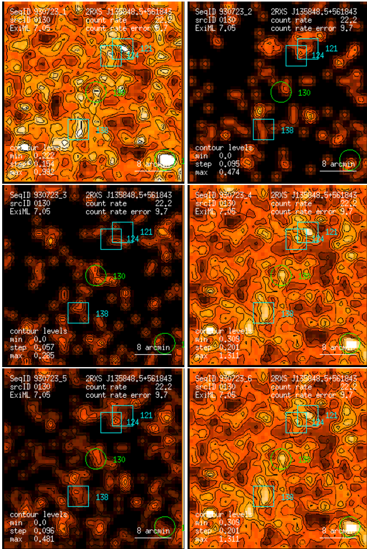
Figure 130: RASS 930723: detection 0130: band rate images, Gaussian filter: (1) PSPC channels 11 – 41, (2) 52 – 90, (3) 91 – 201, (4) 11 – 235, (5) 52 – 201, (6) 11 – 201. Broad band rates in counts/ks. Band rate contour levels in counts/ks/arcmin 2 .
