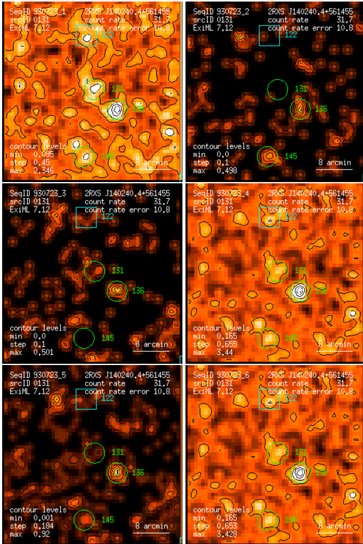
Figure 131: RASS 930723: detection 0131: band rate images, Gaussian filter: (1) PSPC channels 11 – 41, (2) 52 – 90, (3) 91 – 201, (4) 11 – 235, (5) 52 – 201, (6) 11 – 201. Broad band rates in counts/ks. Band rate contour levels in counts/ks/arcmin 2 .
