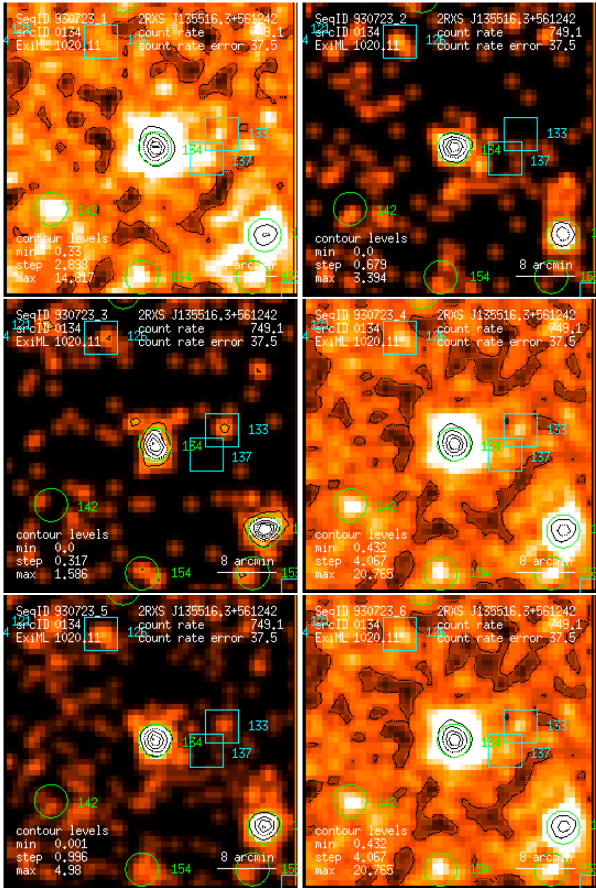
Figure 134: RASS 930723: detection 0134: band rate images, Gaussian filter: (1) PSPC channels 11 – 41, (2) 52 – 90, (3) 91 – 201, (4) 11 – 235, (5) 52 – 201, (6) 11 – 201. Broad band rates in counts/ks. Band rate contour levels in counts/ks/arcmin 2 .
