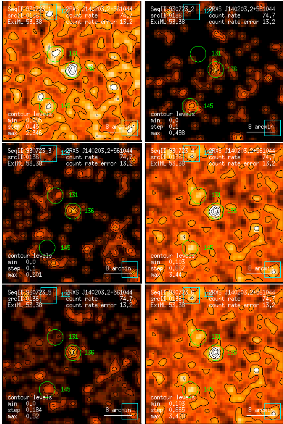
Figure 136: RASS 930723: detection 0136: band rate images, Gaussian filter: (1) PSPC channels 11 – 41, (2) 52 – 90, (3) 91 – 201, (4) 11 – 235, (5) 52 – 201, (6) 11 – 201. Broad band rates in counts/ks. Band rate contour levels in counts/ks/arcmin 2 .
