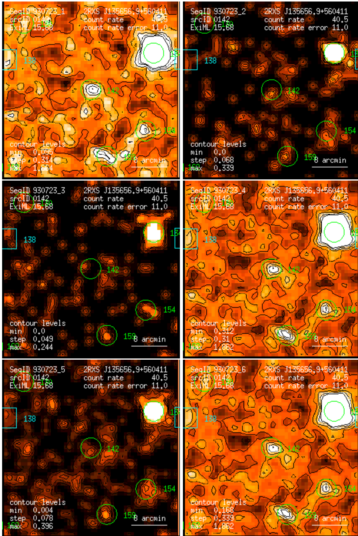
Figure 142: RASS 930723: detection 0142: band rate images, Gaussian filter: (1) PSPC channels 11 – 41, (2) 52 – 90, (3) 91 – 201, (4) 11 – 235, (5) 52 – 201, (6) 11 – 201. Broad band rates in counts/ks. Band rate contour levels in counts/ks/arcmin 2 .
