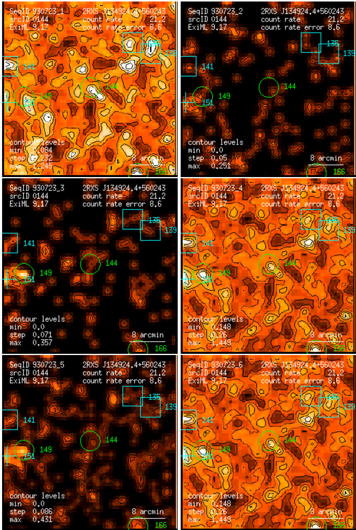
Figure 144: RASS 930723: detection 0144: band rate images, Gaussian filter: (1) PSPC channels 11 – 41, (2) 52 – 90, (3) 91 – 201, (4) 11 – 235, (5) 52 – 201, (6) 11 – 201. Broad band rates in counts/ks. Band rate contour levels in counts/ks/arcmin 2 .
