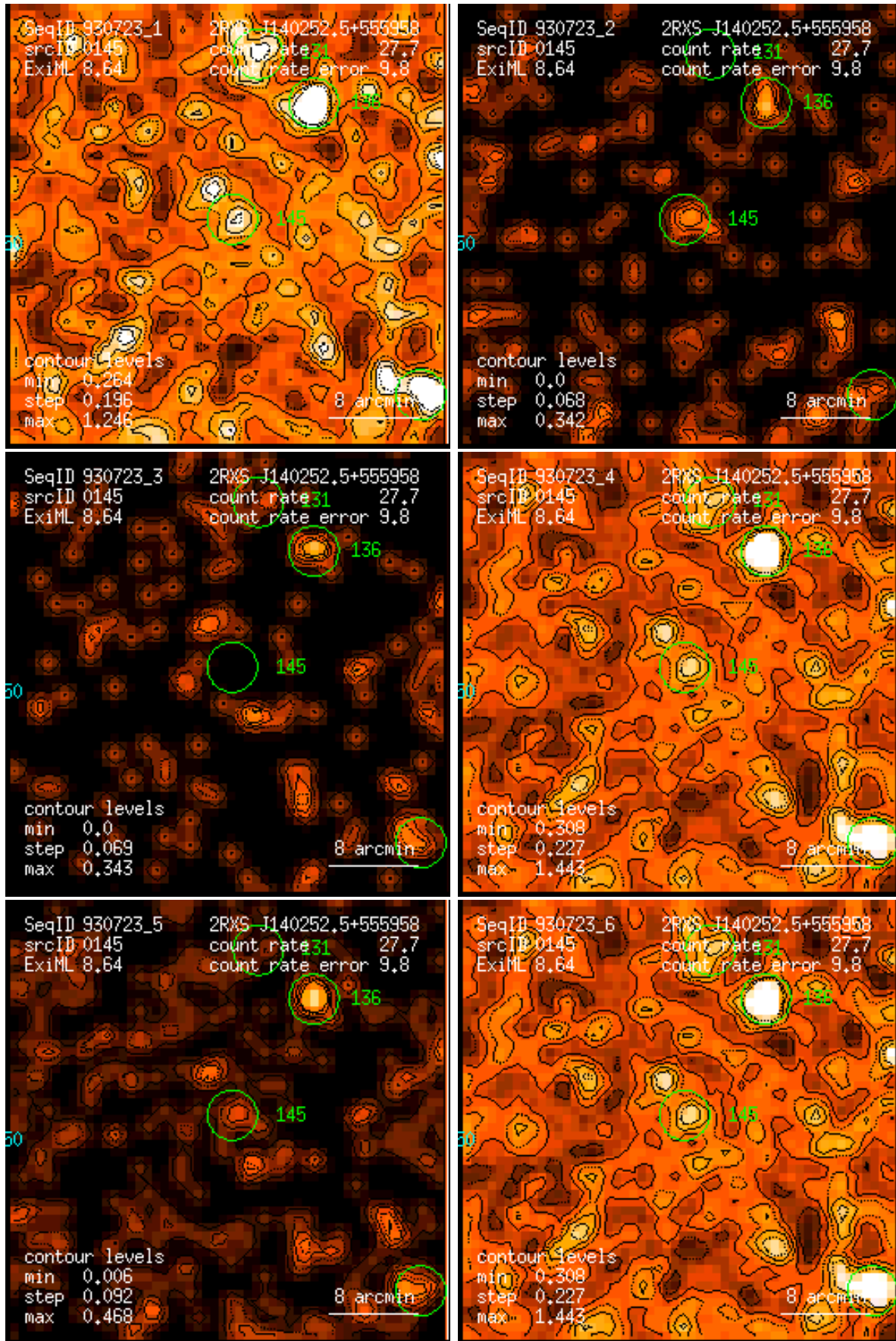
Figure 145: RASS 930723: detection 0145: band rate images, Gaussian filter: (1) PSPC channels 11 – 41, (2) 52 – 90, (3) 91 – 201, (4) 11 – 235, (5) 52 – 201, (6) 11 – 201. Broad band rates in counts/ks. Band rate contour levels in counts/ks/arcmin 2 .
