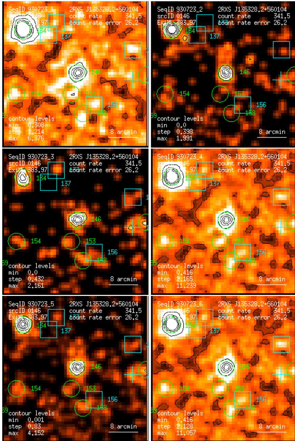
Figure 146: RASS 930723: detection 0146: band rate images, Gaussian filter: (1) PSPC channels 11 – 41, (2) 52 – 90, (3) 91 – 201, (4) 11 – 235, (5) 52 – 201, (6) 11 – 201. Broad band rates in counts/ks. Band rate contour levels in counts/ks/arcmin 2 .
