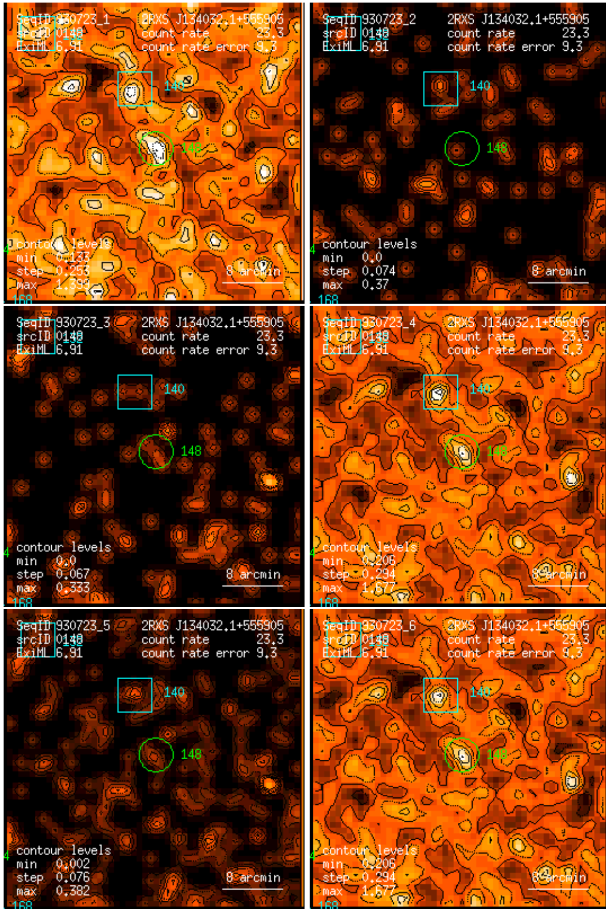
Figure 148: RASS 930723: detection 0148: band rate images, Gaussian filter: (1) PSPC channels 11 – 41, (2) 52 – 90, (3) 91 – 201, (4) 11 – 235, (5) 52 – 201, (6) 11 – 201. Broad band rates in counts/ks. Band rate contour levels in counts/ks/arcmin 2 .
