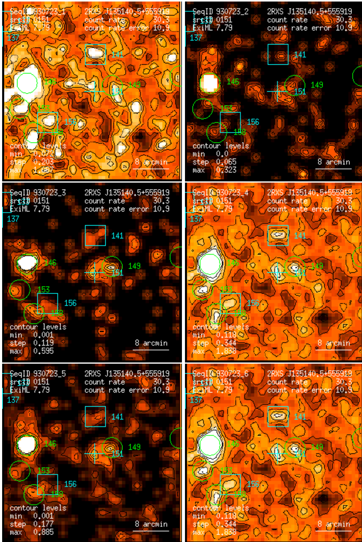
Figure 151: RASS 930723: detection 0151: band rate images, Gaussian filter: (1) PSPC channels 11 – 41, (2) 52 – 90, (3) 91 – 201, (4) 11 – 235, (5) 52 – 201, (6) 11 – 201. Broad band rates in counts/ks. Band rate contour levels in counts/ks/arcmin 2 .
