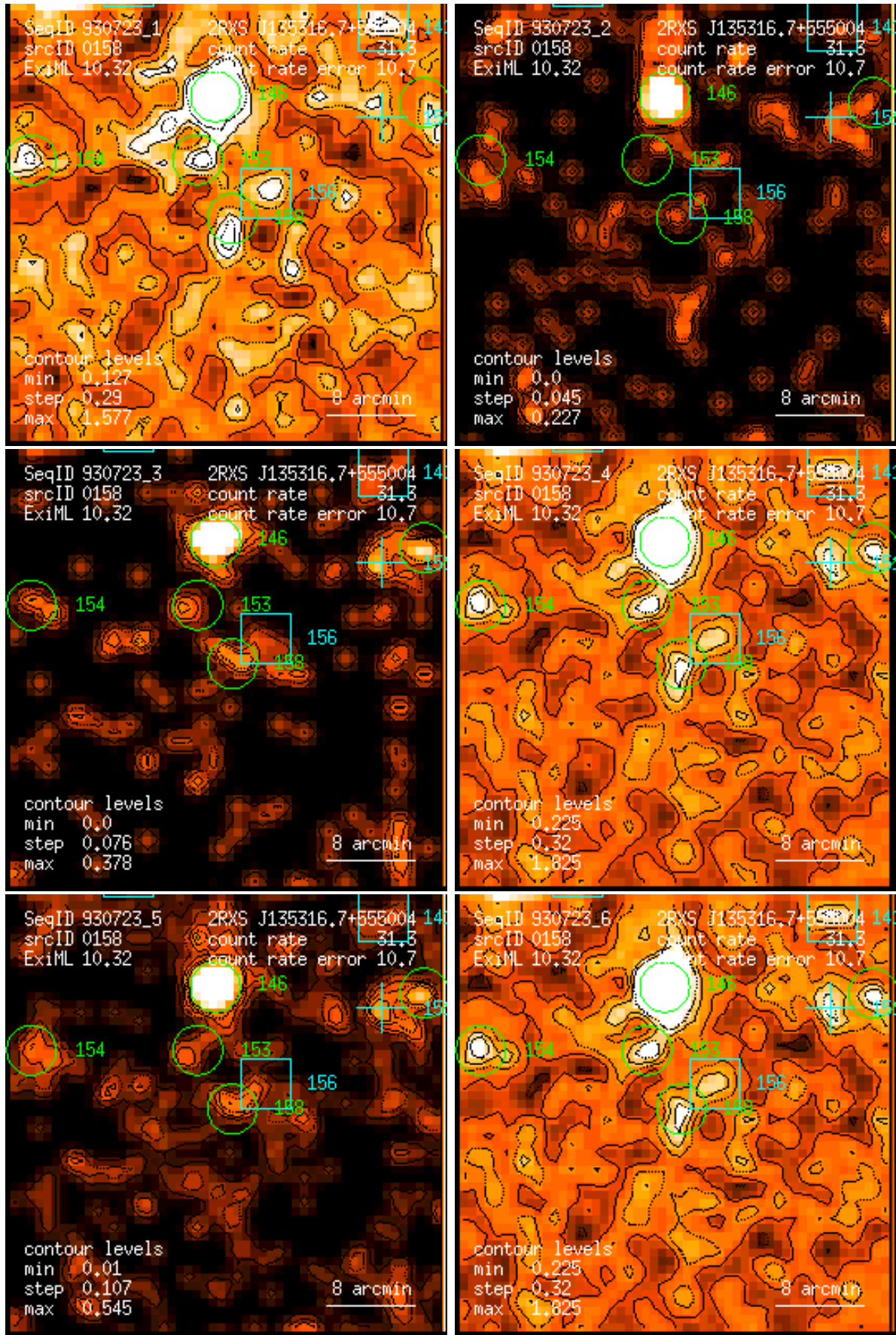
Figure 158: RASS 930723: detection 0158: band rate images, Gaussian filter: (1) PSPC channels 11 – 41, (2) 52 – 90, (3) 91 – 201, (4) 11 – 235, (5) 52 – 201, (6) 11 – 201. Broad band rates in counts/ks. Band rate contour levels in counts/ks/arcmin 2 .
