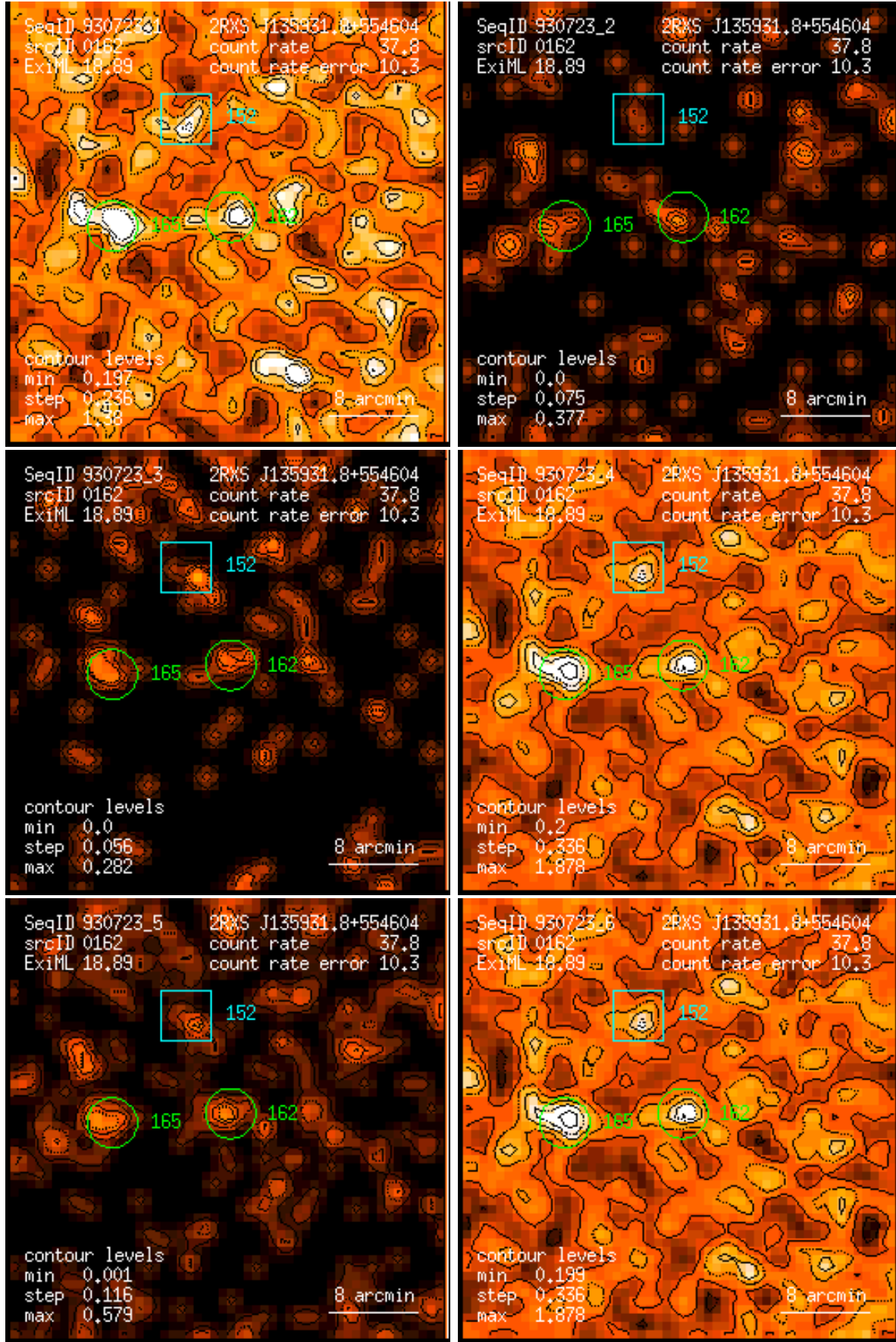
Figure 162: RASS 930723: detection 0162: band rate images, Gaussian filter: (1) PSPC channels 11 – 41, (2) 52 – 90, (3) 91 – 201, (4) 11 – 235, (5) 52 – 201, (6) 11 – 201. Broad band rates in counts/ks. Band rate contour levels in counts/ks/arcmin 2 .
