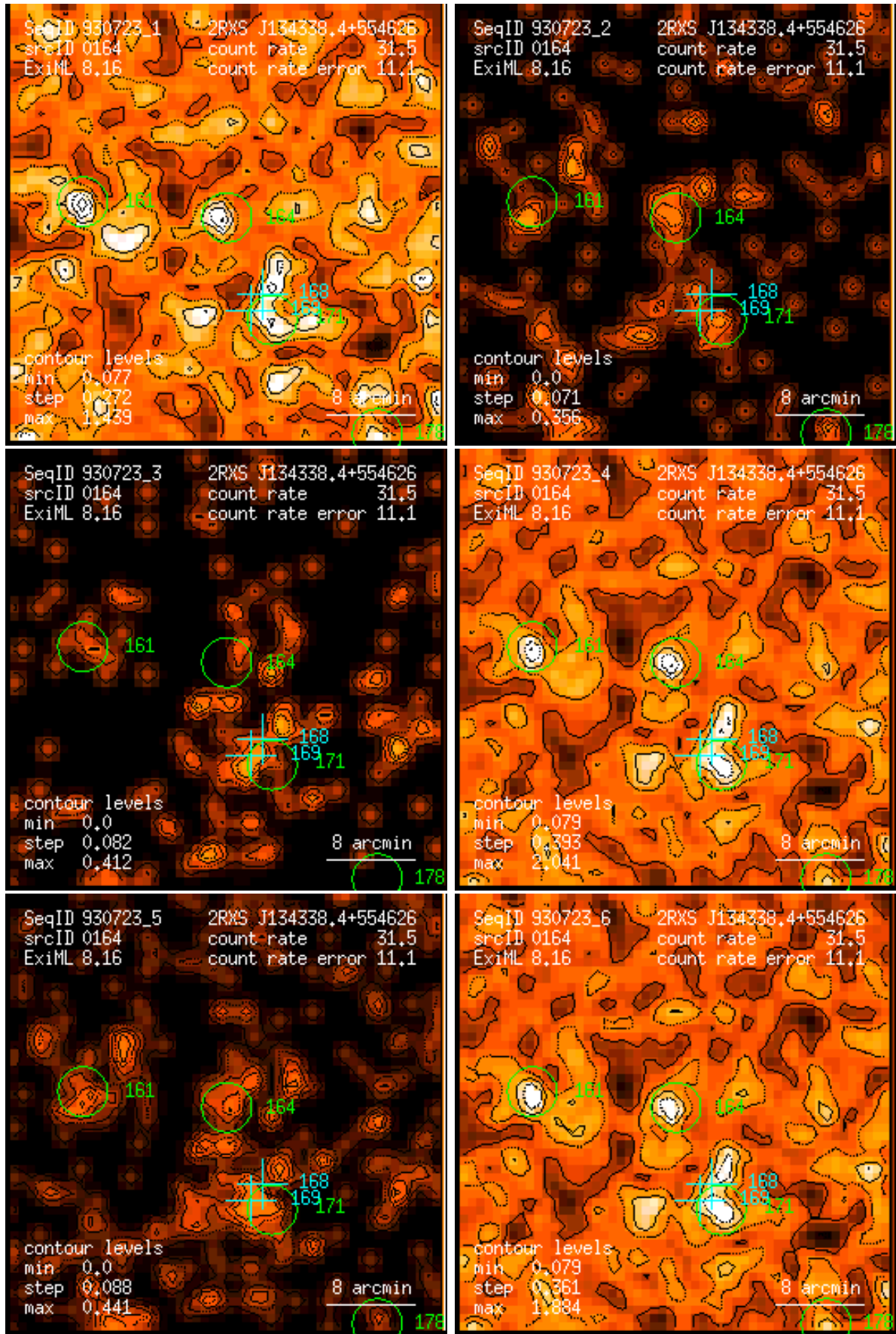
Figure 164: RASS 930723: detection 0164: band rate images, Gaussian filter: (1) PSPC channels 11 – 41, (2) 52 – 90, (3) 91 – 201, (4) 11 – 235, (5) 52 – 201, (6) 11 – 201. Broad band rates in counts/ks. Band rate contour levels in counts/ks/arcmin 2 .
