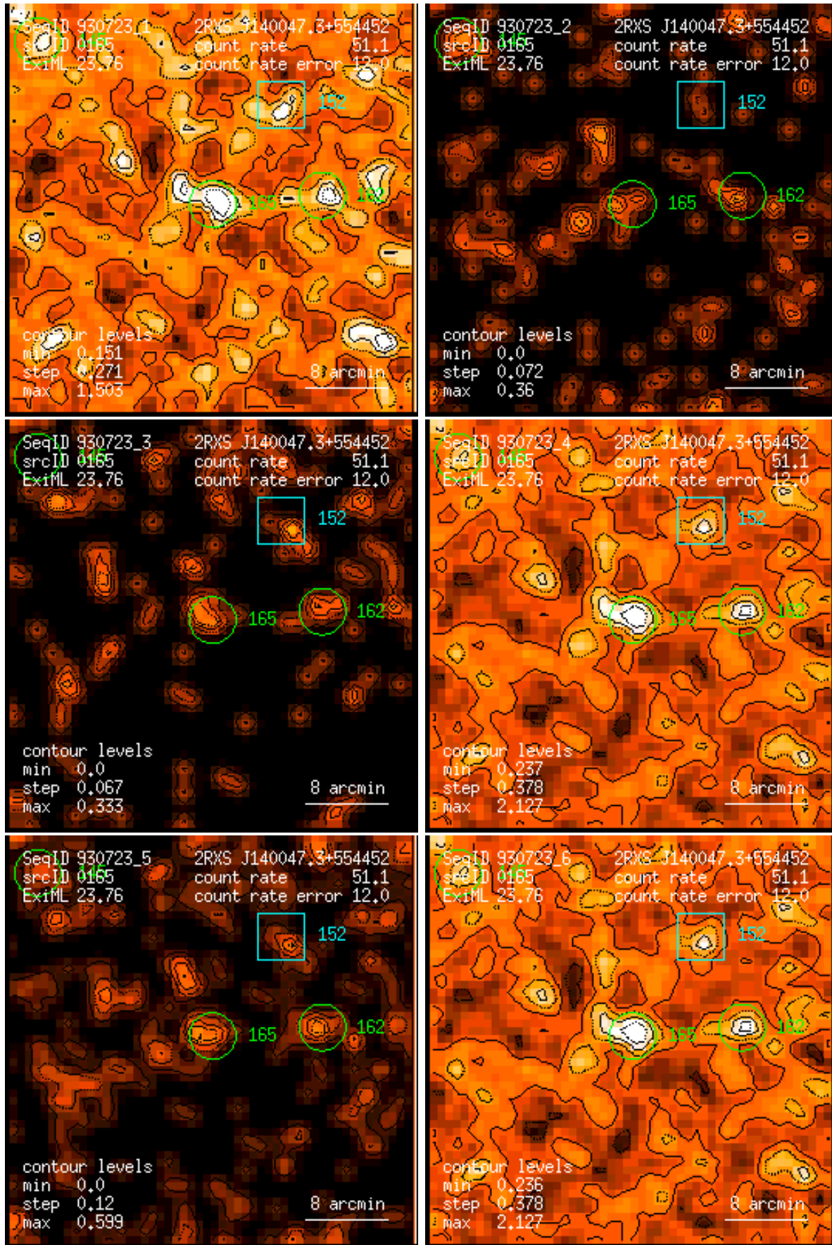
Figure 165: RASS 930723: detection 0165: band rate images, Gaussian filter: (1) PSPC channels 11 – 41, (2) 52 – 90, (3) 91 – 201, (4) 11 – 235, (5) 52 – 201, (6) 11 – 201. Broad band rates in counts/ks. Band rate contour levels in counts/ks/arcmin 2 .
