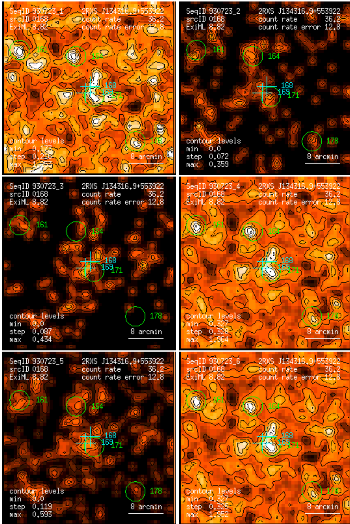
Figure 168: RASS 930723: detection 0168: band rate images, Gaussian filter: (1) PSPC channels 11 – 41, (2) 52 – 90, (3) 91 – 201, (4) 11 – 235, (5) 52 – 201, (6) 11 – 201. Broad band rates in counts/ks. Band rate contour levels in counts/ks/arcmin 2 .
