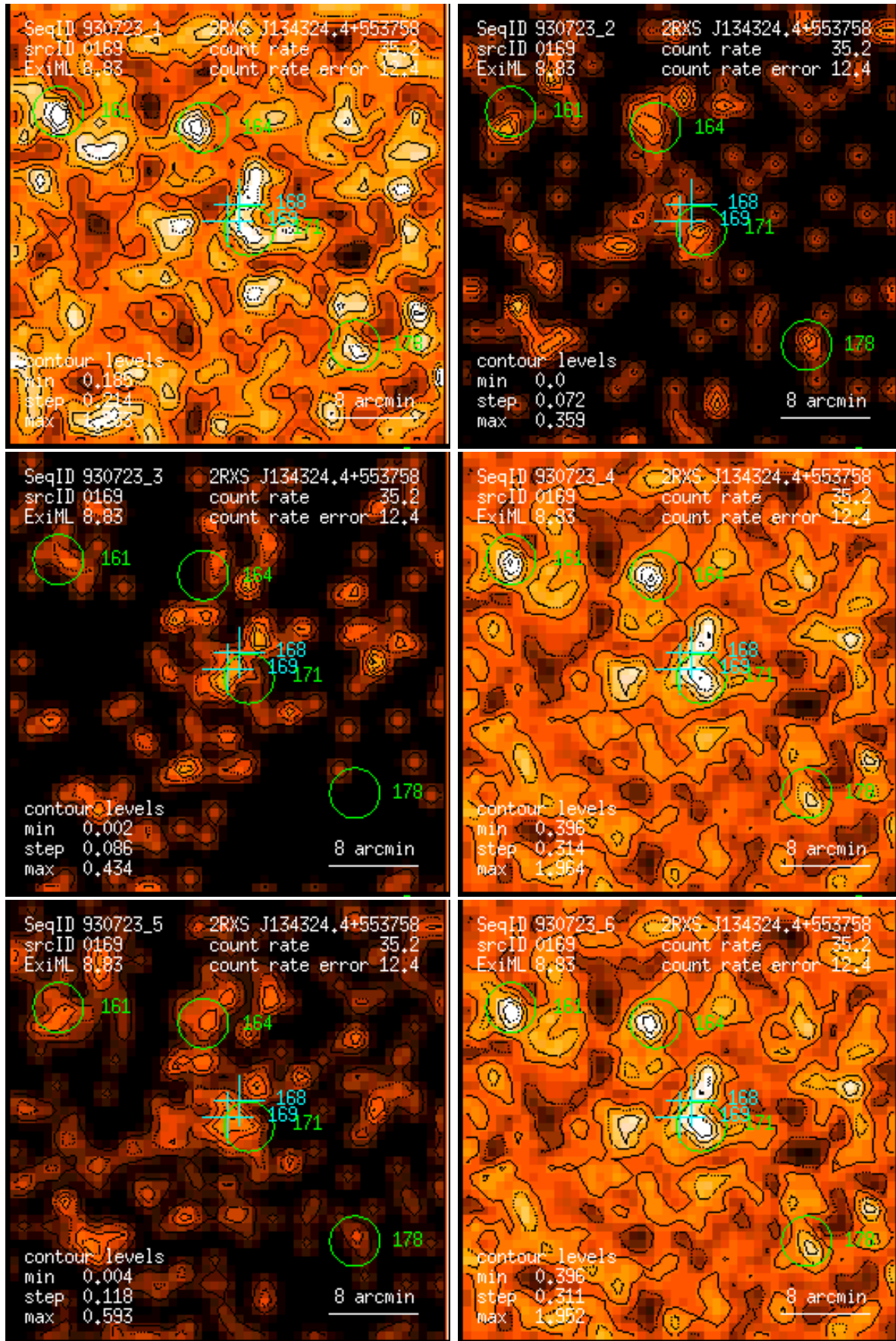
Figure 169: RASS 930723: detection 0169: band rate images, Gaussian filter: (1) PSPC channels 11 – 41, (2) 52 – 90, (3) 91 – 201, (4) 11 – 235, (5) 52 – 201, (6) 11 – 201. Broad band rates in counts/ks. Band rate contour levels in counts/ks/arcmin 2 .
