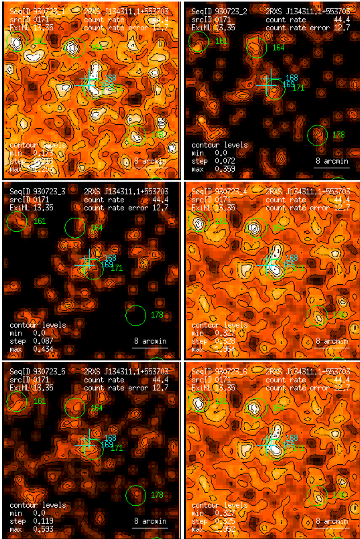
Figure 171: RASS 930723: detection 0171: band rate images, Gaussian filter: (1) PSPC channels 11 – 41, (2) 52 – 90, (3) 91 – 201, (4) 11 – 235, (5) 52 – 201, (6) 11 – 201. Broad band rates in counts/ks. Band rate contour levels in counts/ks/arcmin 2 .
