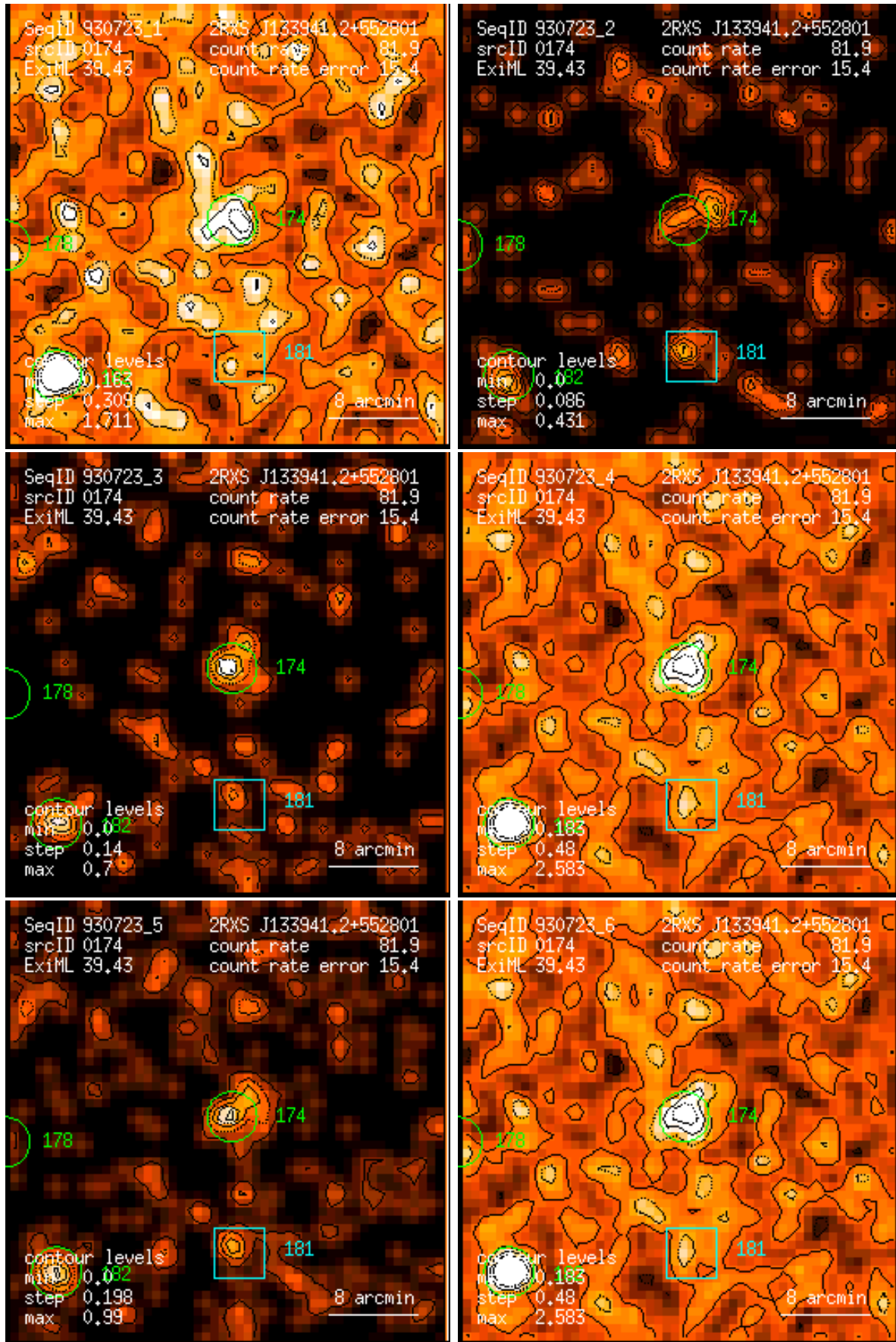
Figure 174: RASS 930723: detection 0174: band rate images, Gaussian filter: (1) PSPC channels 11 – 41, (2) 52 – 90, (3) 91 – 201, (4) 11 – 235, (5) 52 – 201, (6) 11 – 201. Broad band rates in counts/ks. Band rate contour levels in counts/ks/arcmin 2 .
