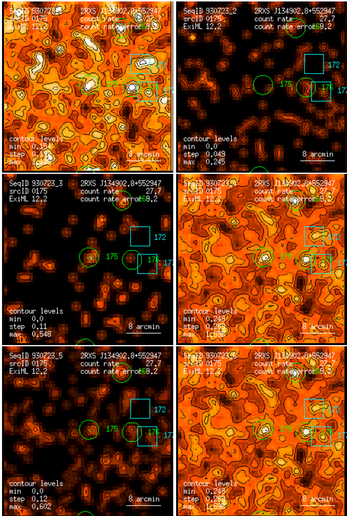
Figure 175: RASS 930723: detection 0175: band rate images, Gaussian filter: (1) PSPC channels 11 – 41, (2) 52 – 90, (3) 91 – 201, (4) 11 – 235, (5) 52 – 201, (6) 11 – 201. Broad band rates in counts/ks. Band rate contour levels in counts/ks/arcmin 2 .
