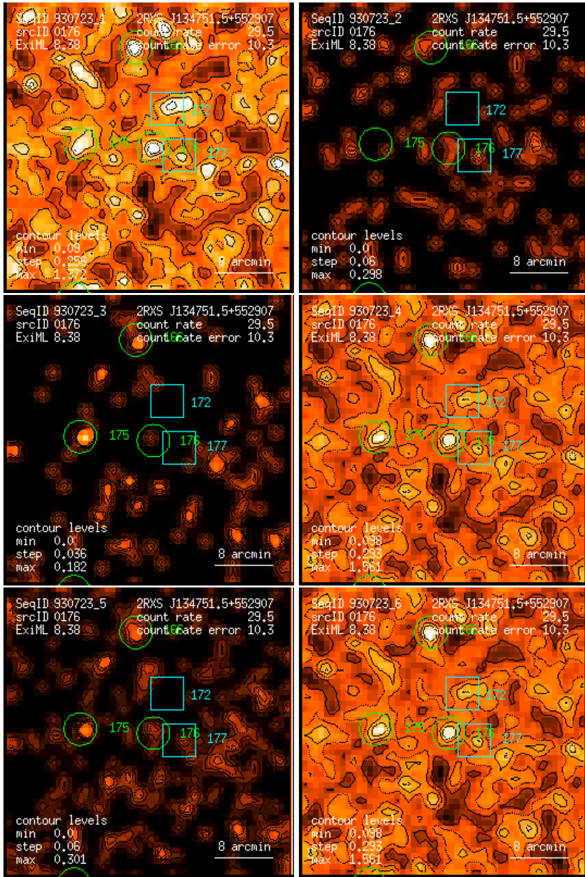
Figure 176: RASS 930723: detection 0176: band rate images, Gaussian filter: (1) PSPC channels 11 – 41, (2) 52 – 90, (3) 91 – 201, (4) 11 – 235, (5) 52 – 201, (6) 11 – 201. Broad band rates in counts/ks. Band rate contour levels in counts/ks/arcmin 2 .
