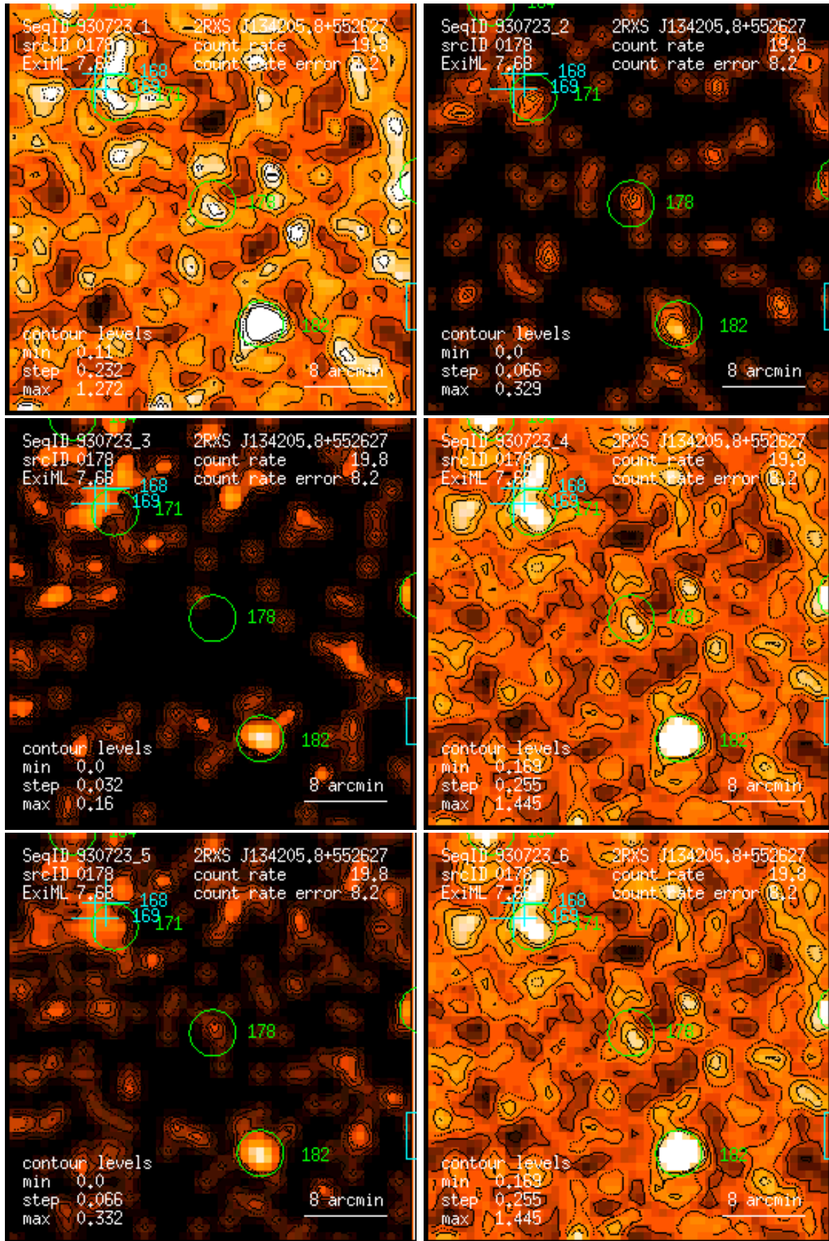
Figure 178: RASS 930723: detection 0178: band rate images, Gaussian filter: (1) PSPC channels 11 – 41, (2) 52 – 90, (3) 91 – 201, (4) 11 – 235, (5) 52 – 201, (6) 11 – 201. Broad band rates in counts/ks. Band rate contour levels in counts/ks/arcmin 2 .
