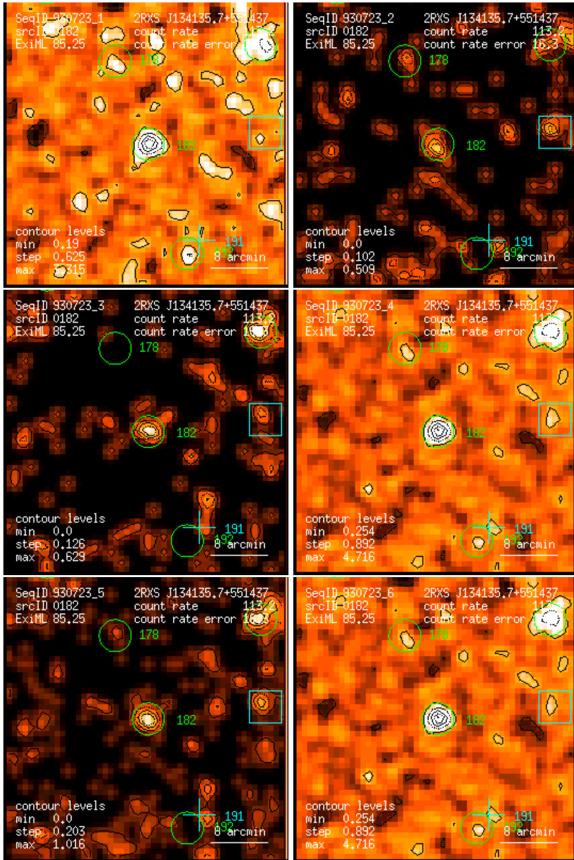
Figure 182: RASS 930723: detection 0182: band rate images, Gaussian filter: (1) PSPC channels 11 – 41, (2) 52 – 90, (3) 91 – 201, (4) 11 – 235, (5) 52 – 201, (6) 11 – 201. Broad band rates in counts/ks. Band rate contour levels in counts/ks/arcmin 2 .
