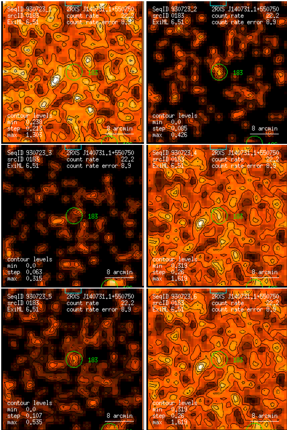
Figure 183: RASS 930723: detection 0183: band rate images, Gaussian filter: (1) PSPC channels 11 – 41, (2) 52 – 90, (3) 91 – 201, (4) 11 – 235, (5) 52 – 201, (6) 11 – 201. Broad band rates in counts/ks. Band rate contour levels in counts/ks/arcmin 2 .
