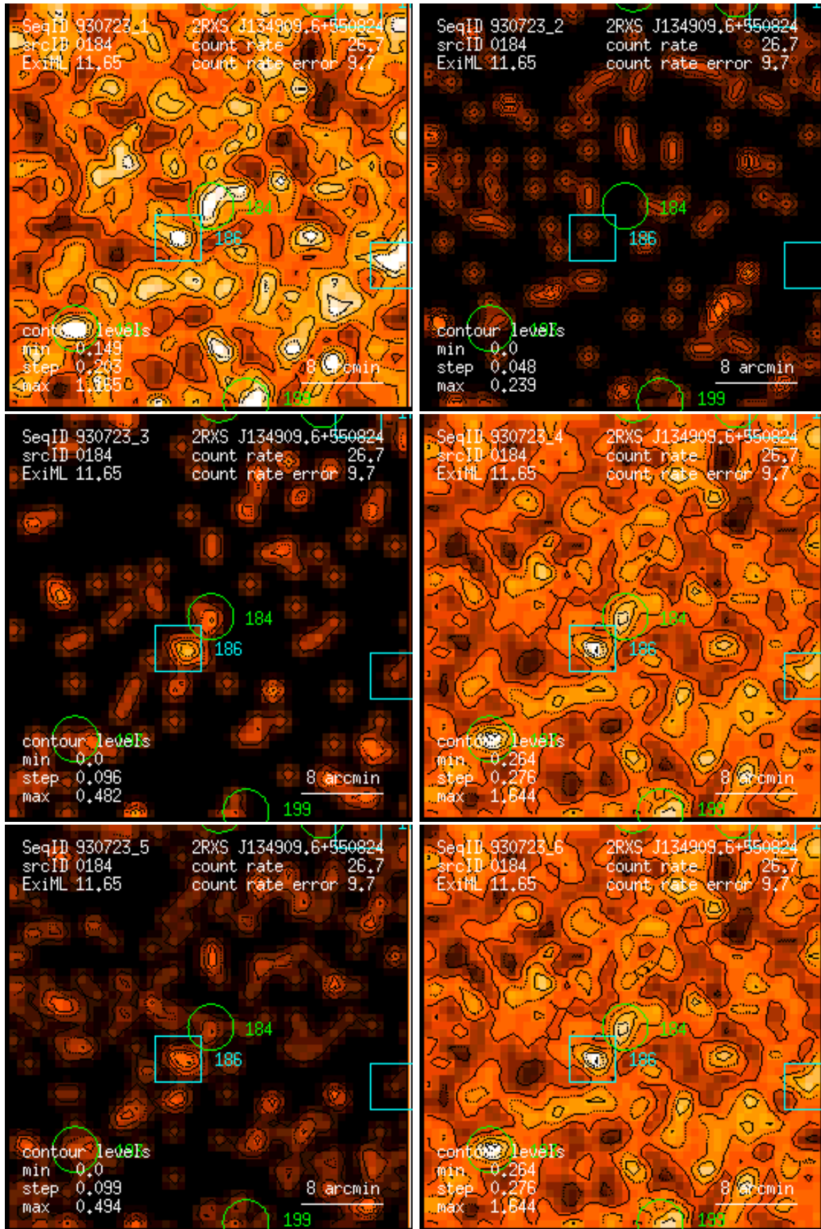
Figure 184: RASS 930723: detection 0184: band rate images, Gaussian filter: (1) PSPC channels 11 – 41, (2) 52 – 90, (3) 91 – 201, (4) 11 – 235, (5) 52 – 201, (6) 11 – 201. Broad band rates in counts/ks. Band rate contour levels in counts/ks/arcmin 2 .
