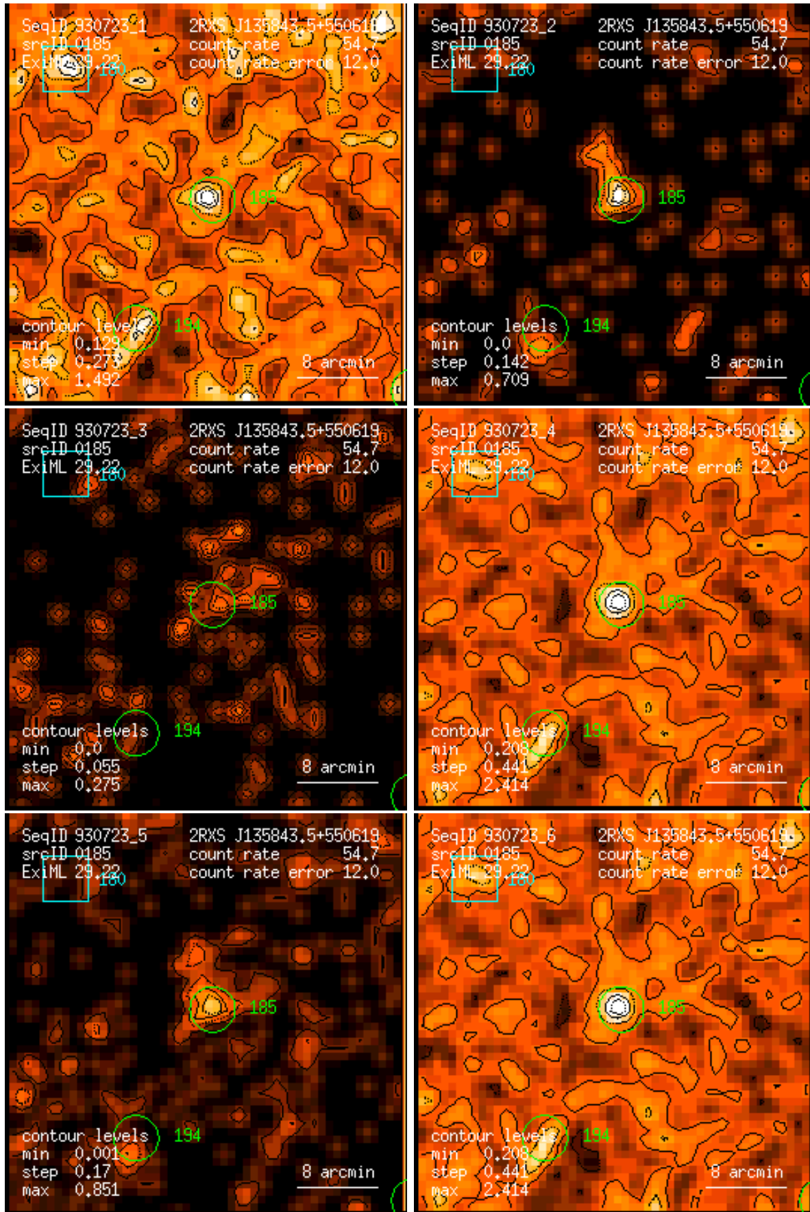
Figure 185: RASS 930723: detection 0185: band rate images, Gaussian filter: (1) PSPC channels 11 – 41, (2) 52 – 90, (3) 91 – 201, (4) 11 – 235, (5) 52 – 201, (6) 11 – 201. Broad band rates in counts/ks. Band rate contour levels in counts/ks/arcmin 2 .
