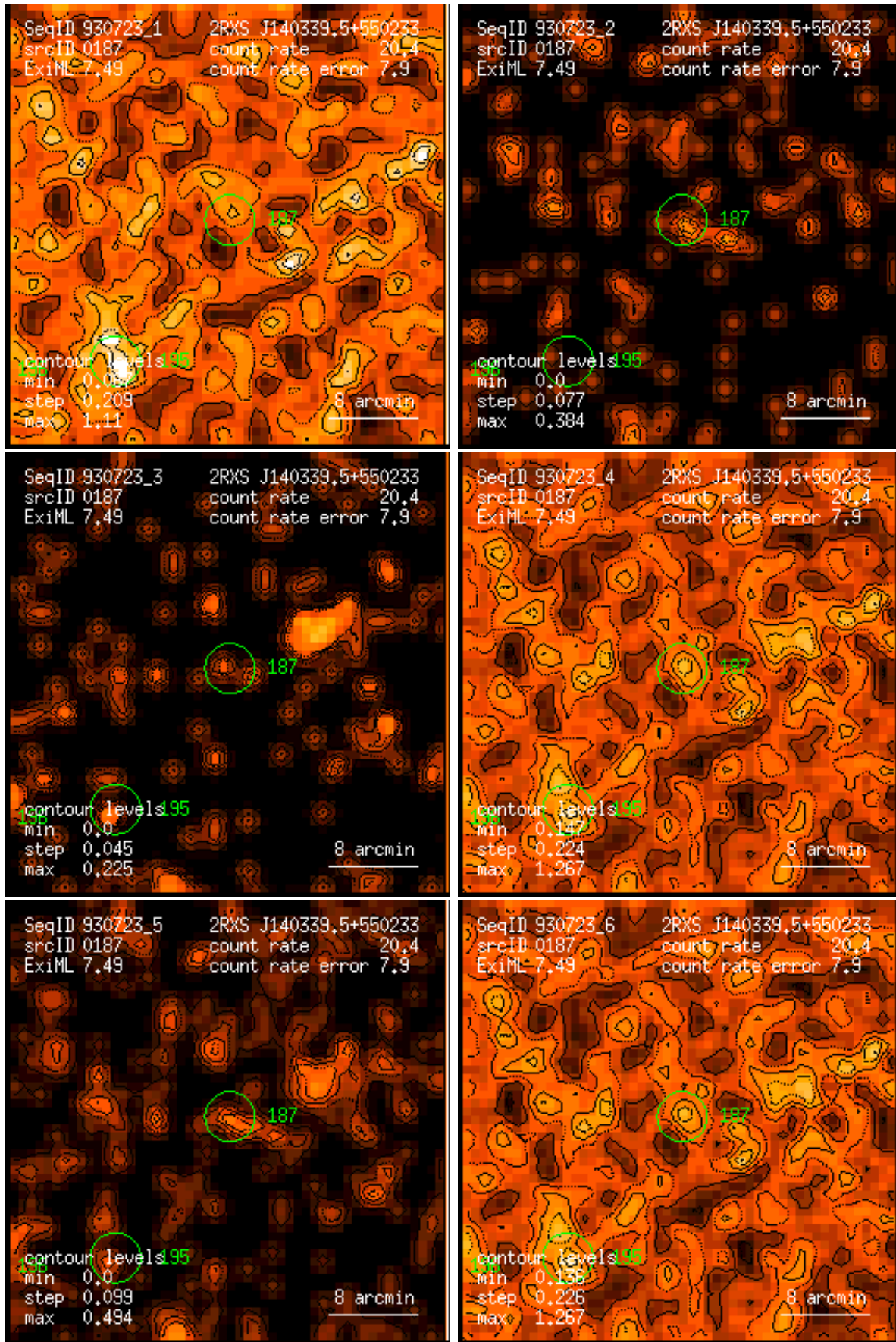
Figure 187: RASS 930723: detection 0187: band rate images, Gaussian filter: (1) PSPC channels 11 – 41, (2) 52 – 90, (3) 91 – 201, (4) 11 – 235, (5) 52 – 201, (6) 11 – 201. Broad band rates in counts/ks. Band rate contour levels in counts/ks/arcmin 2 .
