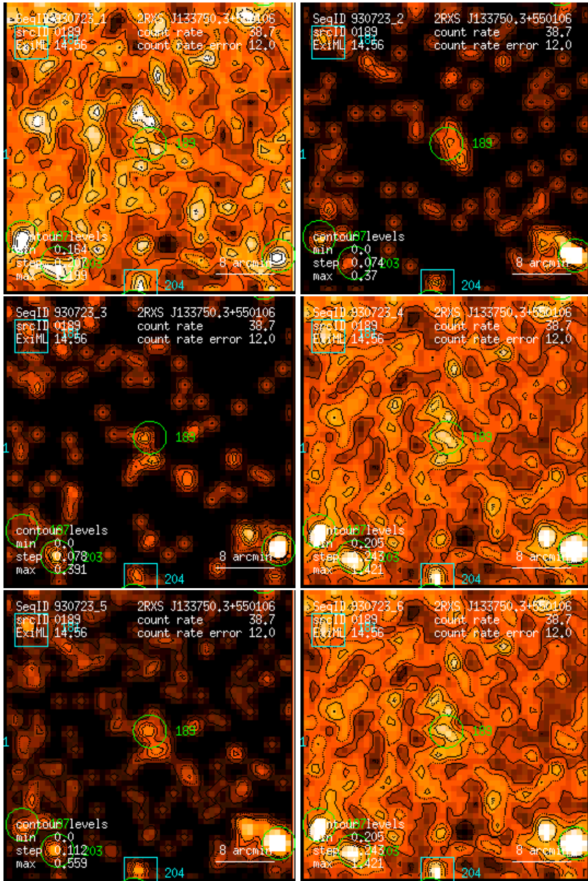
Figure 189: RASS 930723: detection 0189: band rate images, Gaussian filter: (1) PSPC channels 11 – 41, (2) 52 – 90, (3) 91 – 201, (4) 11 – 235, (5) 52 – 201, (6) 11 – 201. Broad band rates in counts/ks. Band rate contour levels in counts/ks/arcmin 2 .
