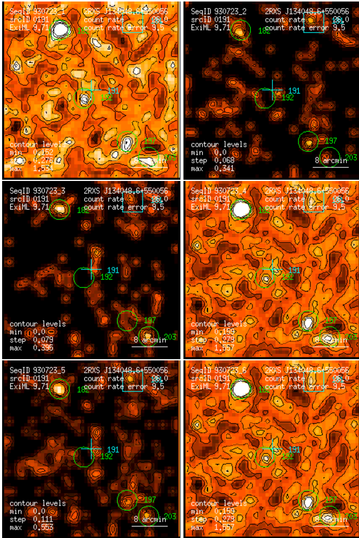
Figure 191: RASS 930723: detection 0191: band rate images, Gaussian filter: (1) PSPC channels 11 – 41, (2) 52 – 90, (3) 91 – 201, (4) 11 – 235, (5) 52 – 201, (6) 11 – 201. Broad band rates in counts/ks. Band rate contour levels in counts/ks/arcmin 2 .
