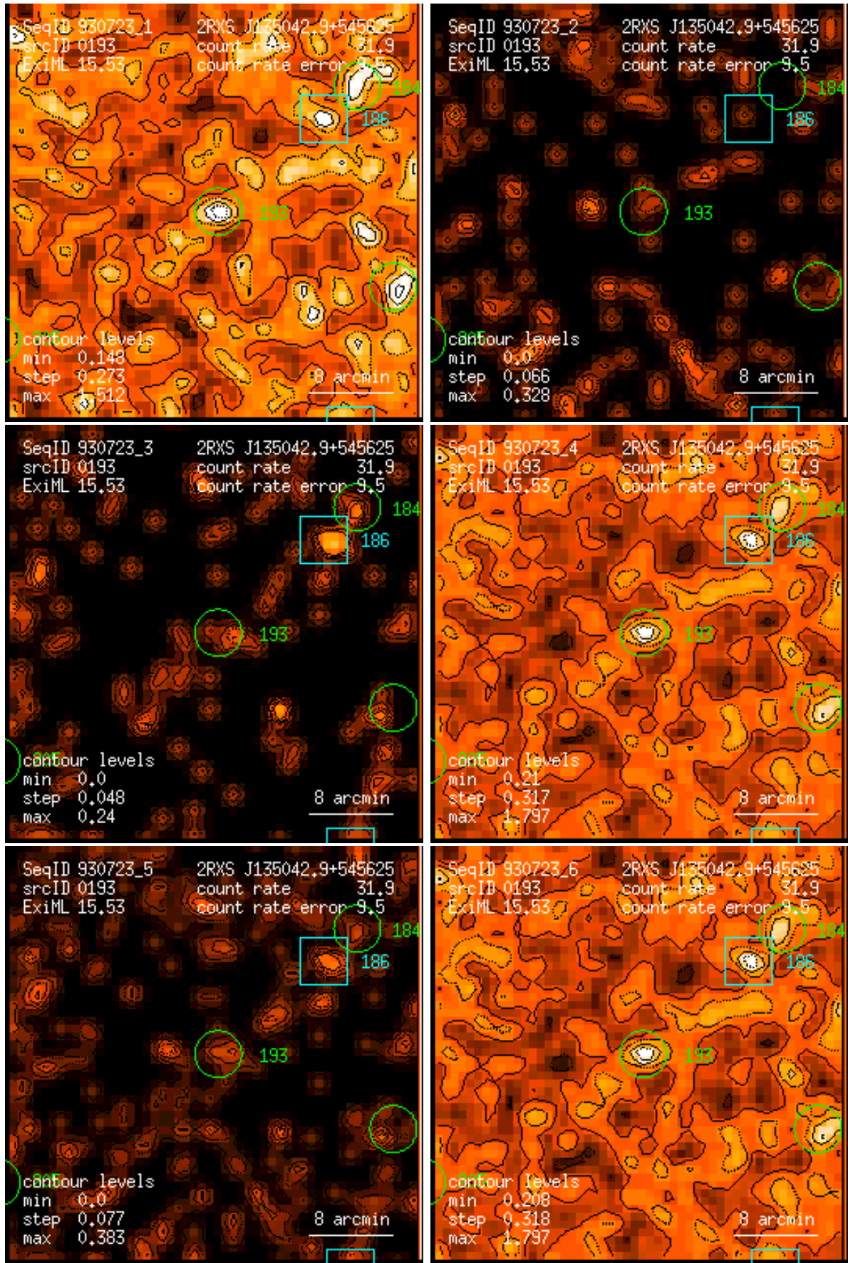
Figure 193: RASS 930723: detection 0193: band rate images, Gaussian filter: (1) PSPC channels 11 – 41, (2) 52 – 90, (3) 91 – 201, (4) 11 – 235, (5) 52 – 201, (6) 11 – 201. Broad band rates in counts/ks. Band rate contour levels in counts/ks/arcmin 2 .
