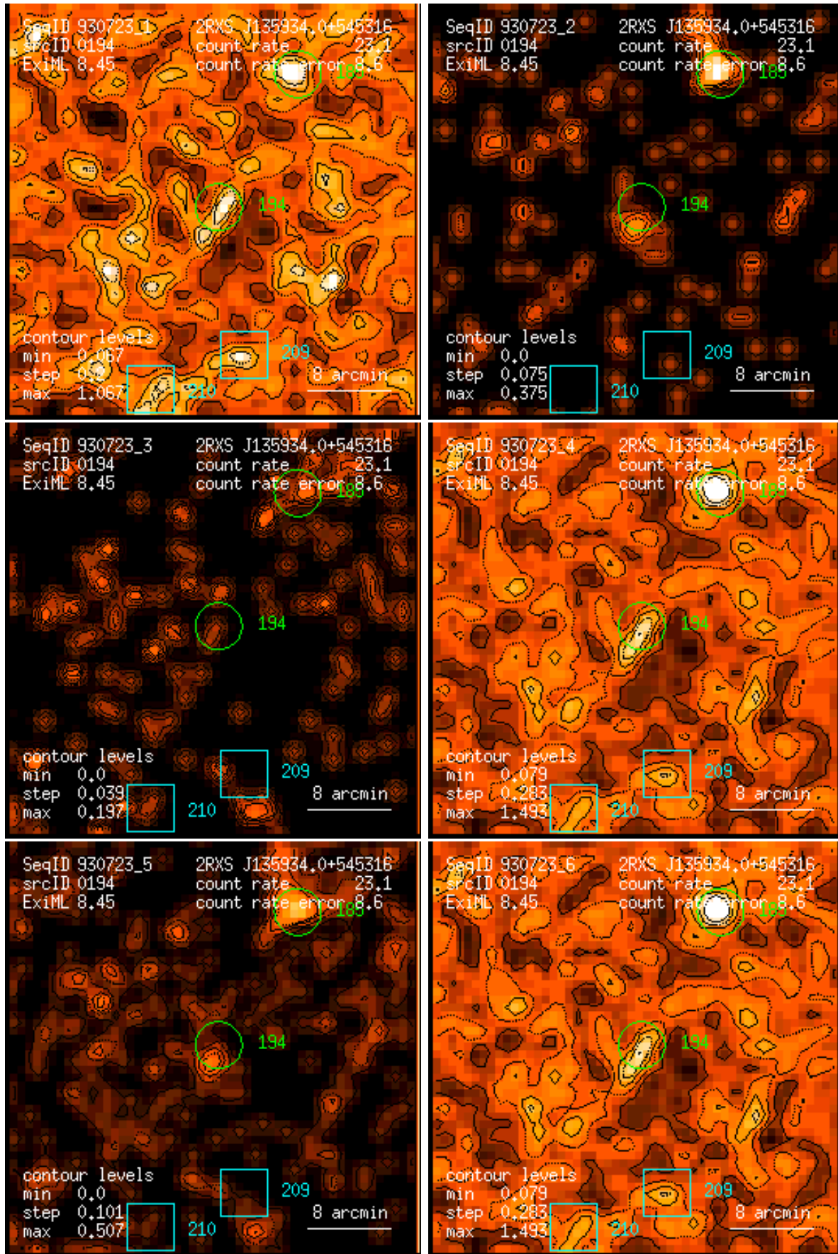
Figure 194: RASS 930723: detection 0194: band rate images, Gaussian filter: (1) PSPC channels 11 – 41, (2) 52 – 90, (3) 91 – 201, (4) 11 – 235, (5) 52 – 201, (6) 11 – 201. Broad band rates in counts/ks. Band rate contour levels in counts/ks/arcmin 2 .
