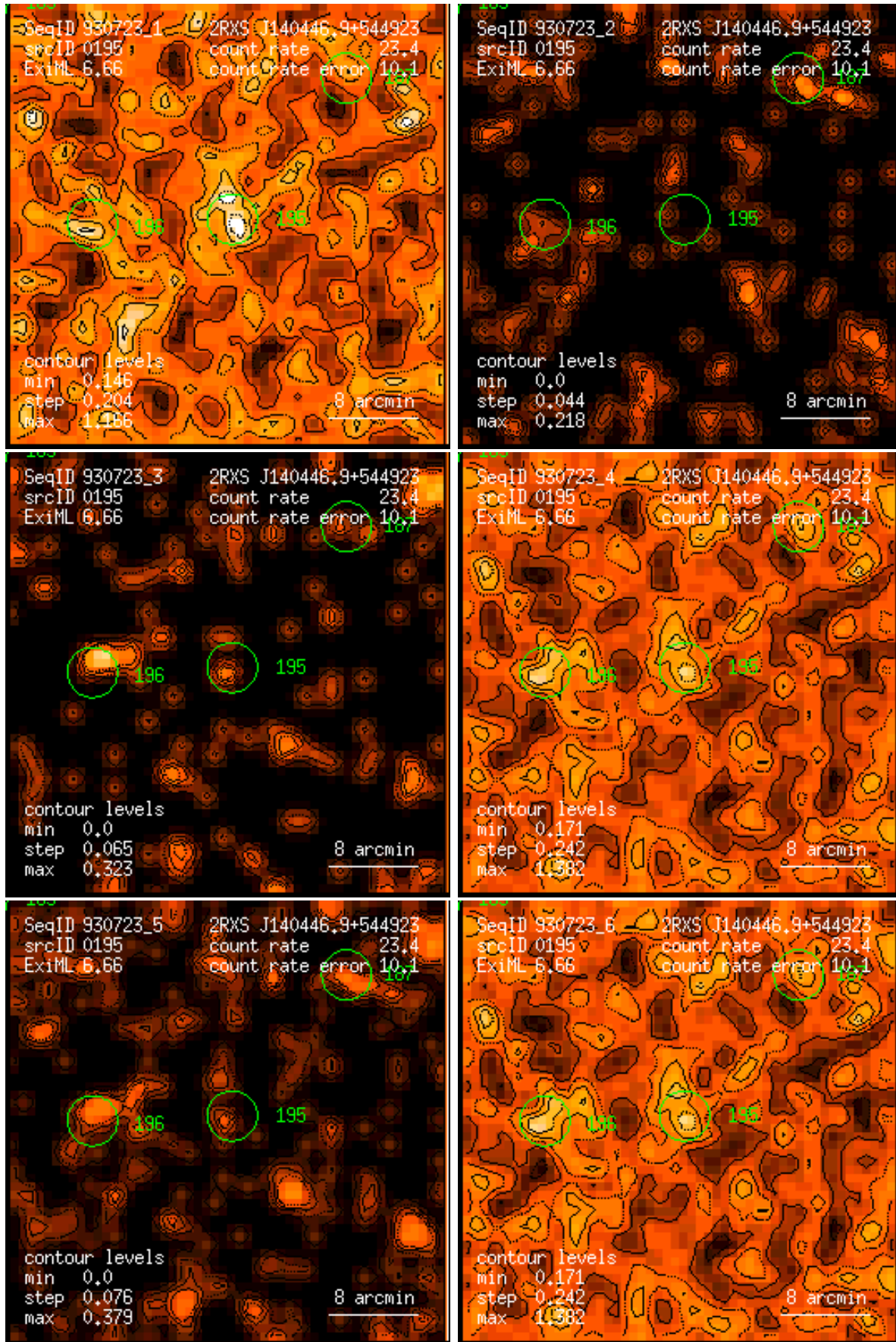
Figure 195: RASS 930723: detection 0195: band rate images, Gaussian filter: (1) PSPC channels 11 – 41, (2) 52 – 90, (3) 91 – 201, (4) 11 – 235, (5) 52 – 201, (6) 11 – 201. Broad band rates in counts/ks. Band rate contour levels in counts/ks/arcmin 2 .
