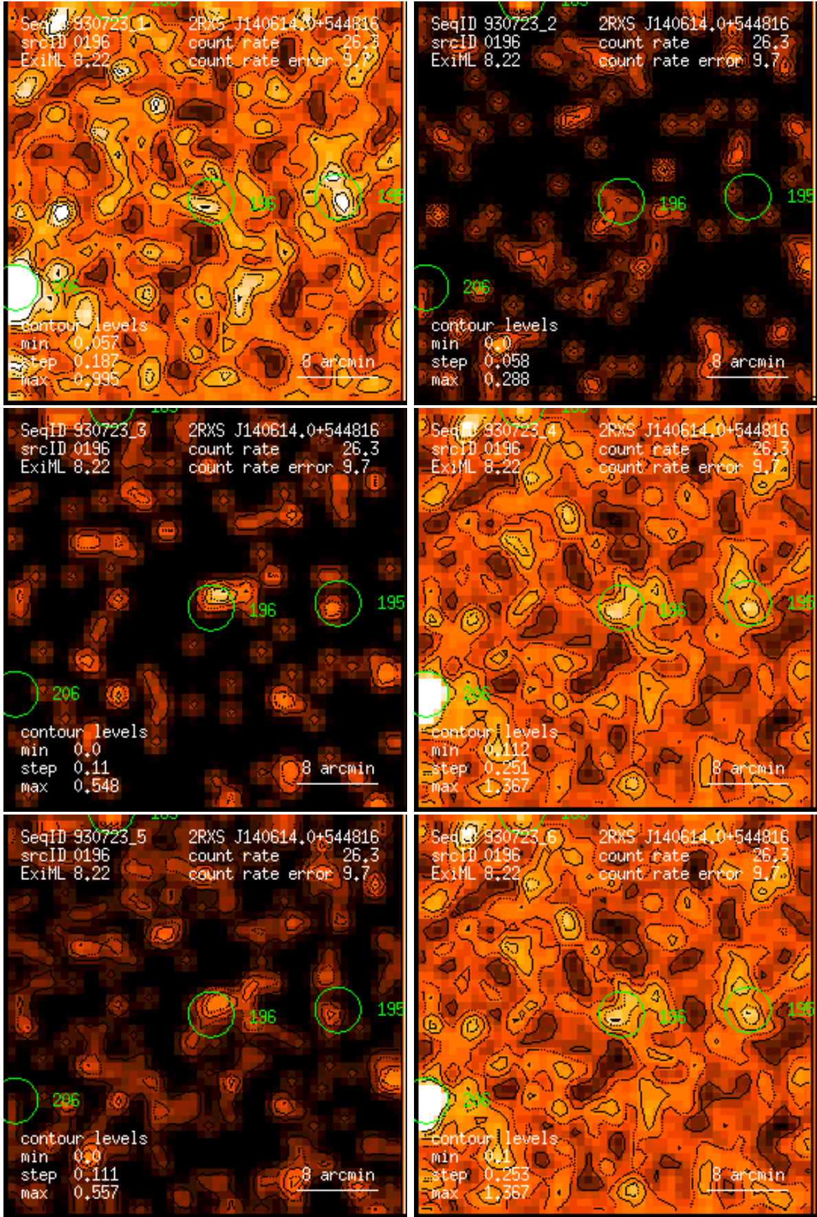
Figure 196: RASS 930723: detection 0196: band rate images, Gaussian filter: (1) PSPC channels 11 – 41, (2) 52 – 90, (3) 91 – 201, (4) 11 – 235, (5) 52 – 201, (6) 11 – 201. Broad band rates in counts/ks. Band rate contour levels in counts/ks/arcmin 2 .
