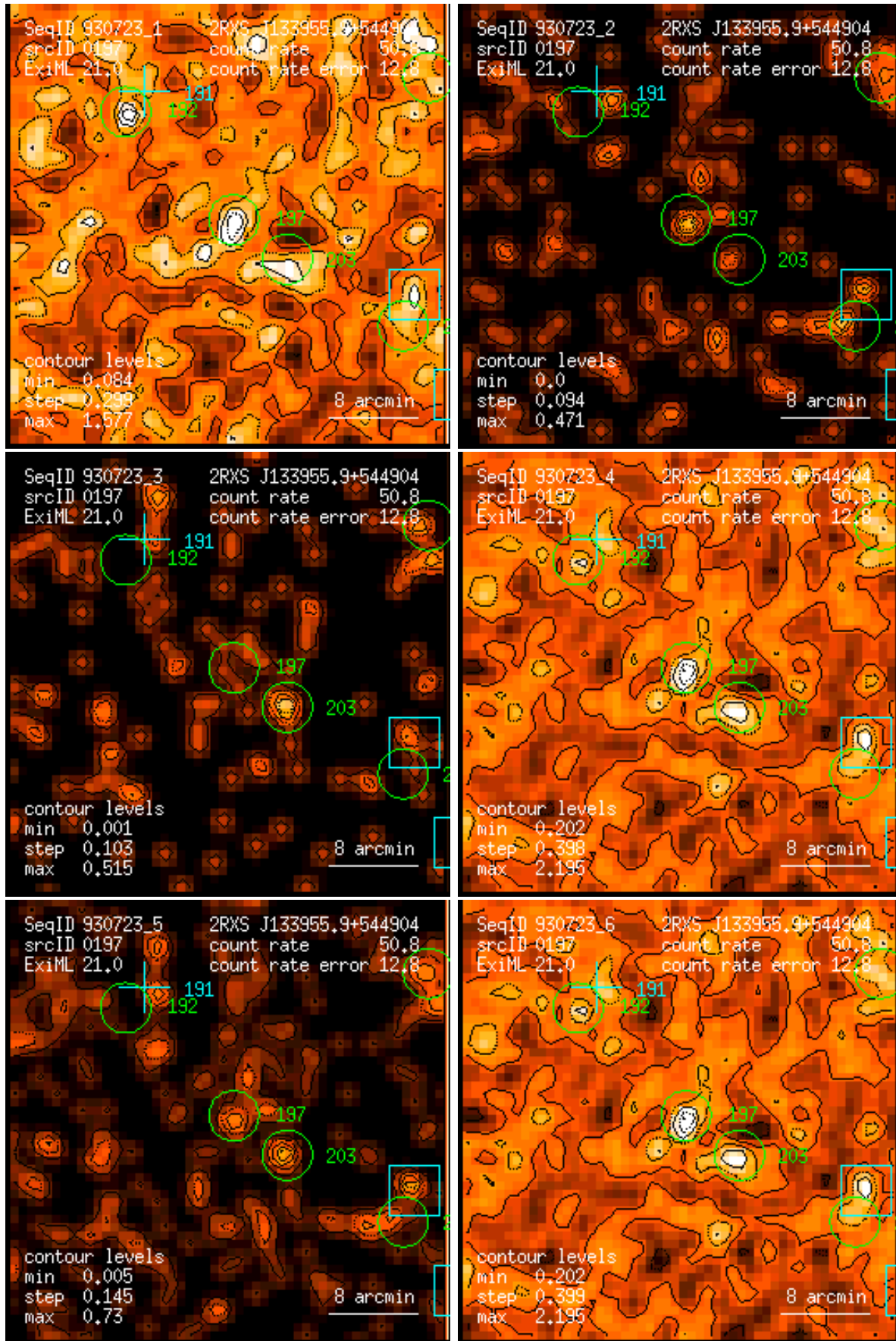
Figure 197: RASS 930723: detection 0197: band rate images, Gaussian filter: (1) PSPC channels 11 – 41, (2) 52 – 90, (3) 91 – 201, (4) 11 – 235, (5) 52 – 201, (6) 11 – 201. Broad band rates in counts/ks. Band rate contour levels in counts/ks/arcmin 2 .
