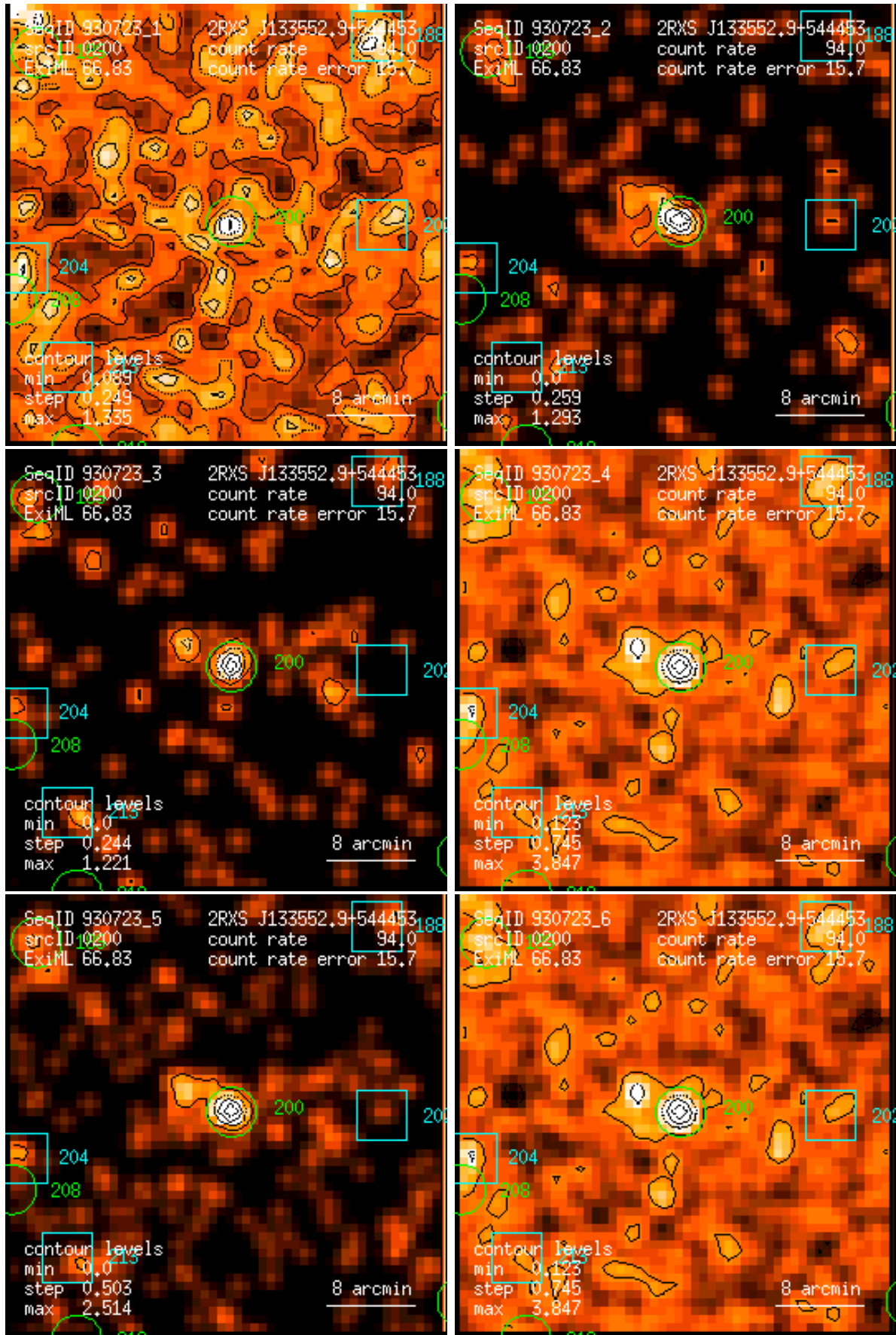
Figure 200: RASS 930723: detection 0200: band rate images, Gaussian filter: (1) PSPC channels 11 – 41, (2) 52 – 90, (3) 91 – 201, (4) 11 – 235, (5) 52 – 201, (6) 11 – 201. Broad band rates in counts/ks. Band rate contour levels in counts/ks/arcmin 2 .
