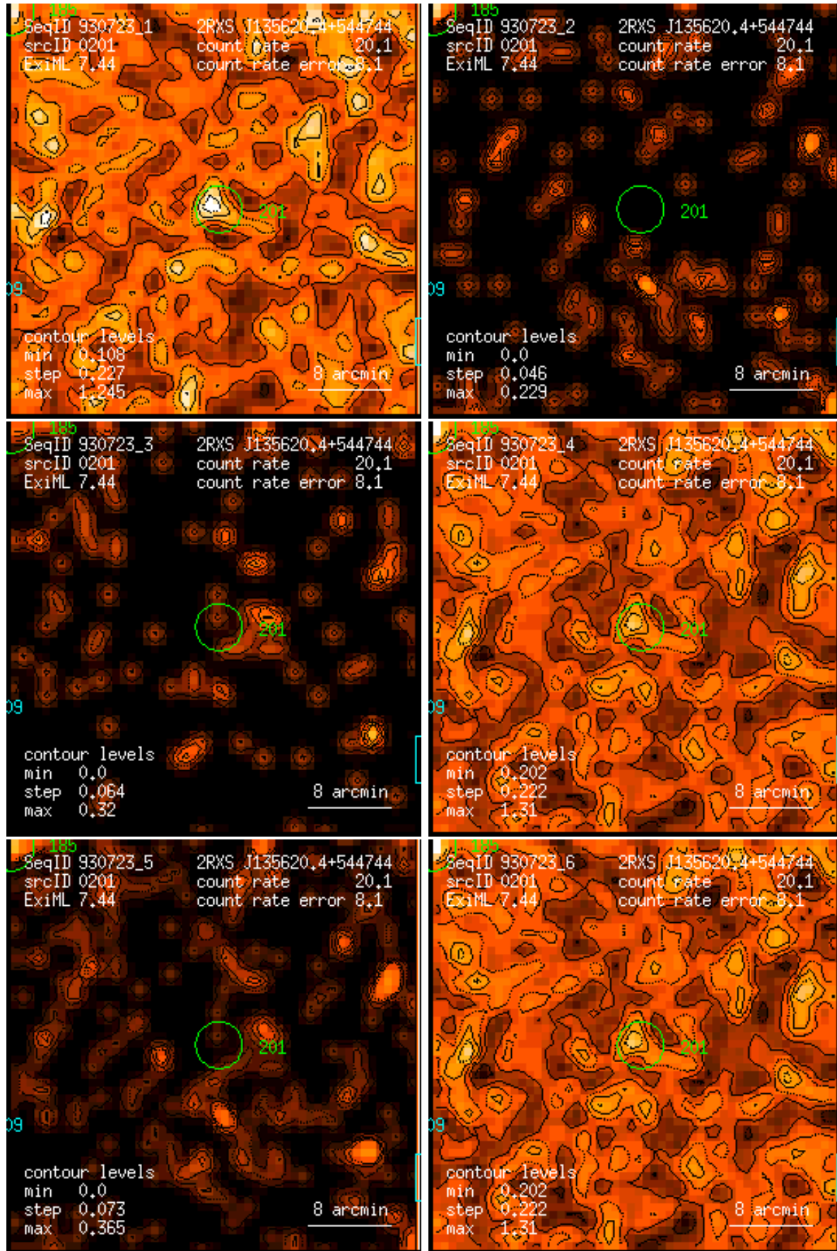
Figure 201: RASS 930723: detection 0201: band rate images, Gaussian filter: (1) PSPC channels 11 – 41, (2) 52 – 90, (3) 91 – 201, (4) 11 – 235, (5) 52 – 201, (6) 11 – 201. Broad band rates in counts/ks. Band rate contour levels in counts/ks/arcmin 2 .
