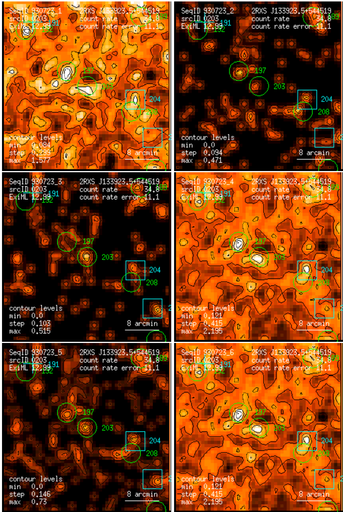
Figure 203: RASS 930723: detection 0203: band rate images, Gaussian filter: (1) PSPC channels 11 – 41, (2) 52 – 90, (3) 91 – 201, (4) 11 – 235, (5) 52 – 201, (6) 11 – 201. Broad band rates in counts/ks. Band rate contour levels in counts/ks/arcmin 2 .
