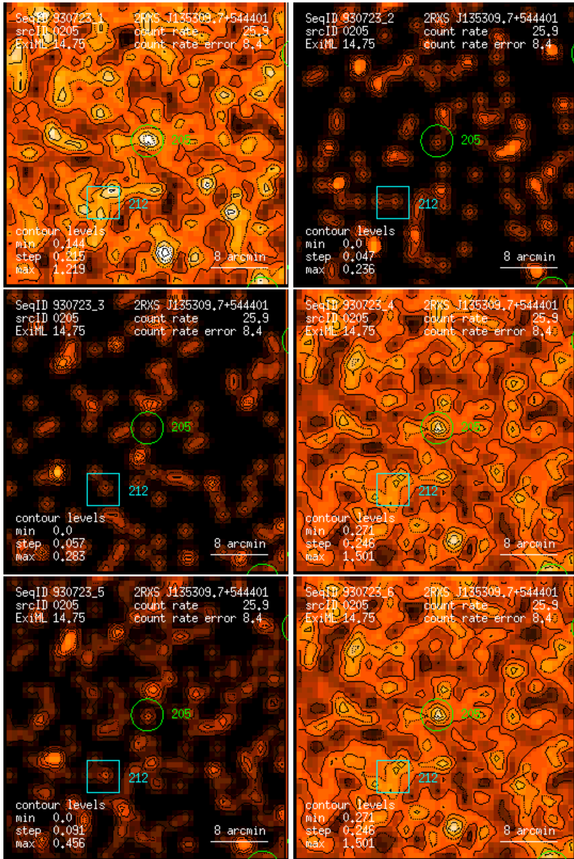
Figure 205: RASS 930723: detection 0205: band rate images, Gaussian filter: (1) PSPC channels 11 – 41, (2) 52 – 90, (3) 91 – 201, (4) 11 – 235, (5) 52 – 201, (6) 11 – 201. Broad band rates in counts/ks. Band rate contour levels in counts/ks/arcmin 2 .
