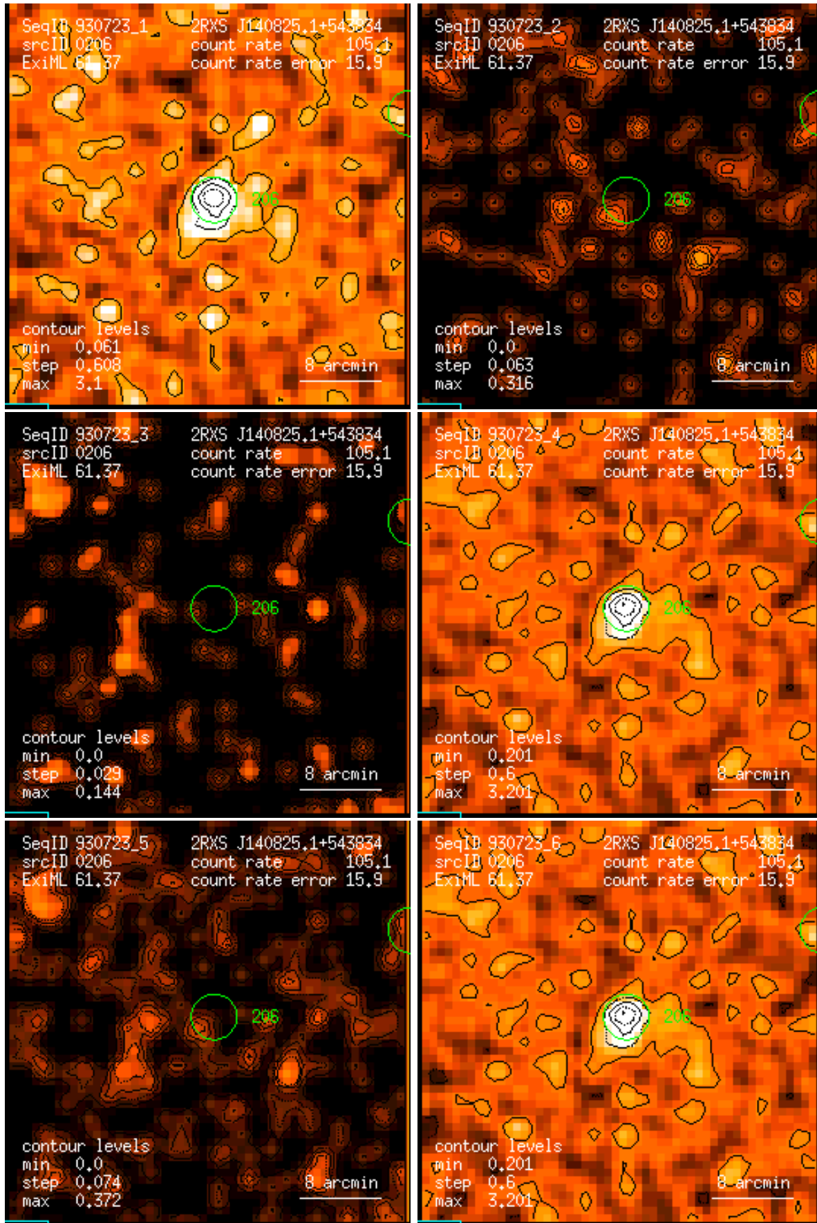
Figure 206: RASS 930723: detection 0206: band rate images, Gaussian filter: (1) PSPC channels 11 – 41, (2) 52 – 90, (3) 91 – 201, (4) 11 – 235, (5) 52 – 201, (6) 11 – 201. Broad band rates in counts/ks. Band rate contour levels in counts/ks/arcmin 2 .
