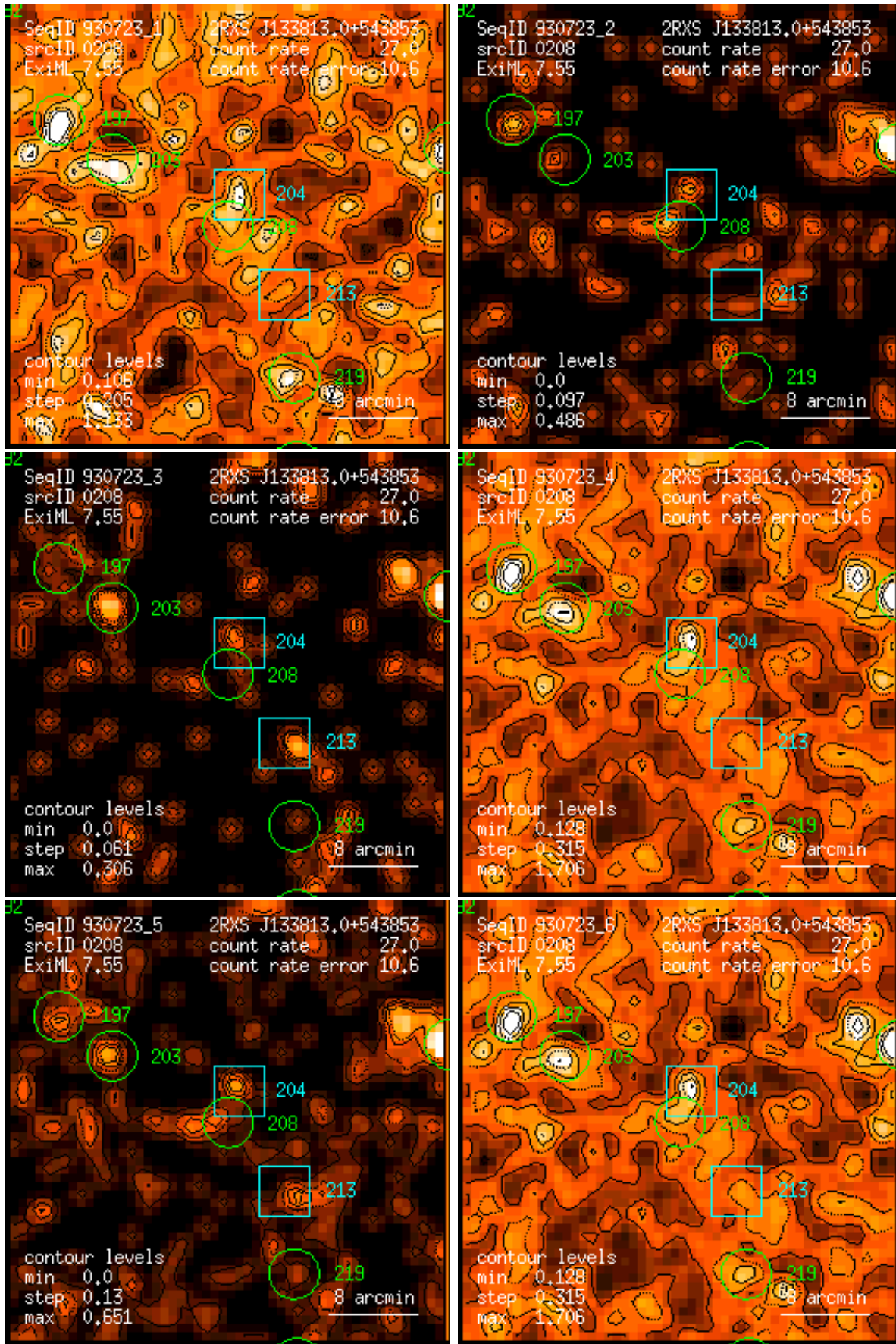
Figure 208: RASS 930723: detection 0208: band rate images, Gaussian filter: (1) PSPC channels 11 – 41, (2) 52 – 90, (3) 91 – 201, (4) 11 – 235, (5) 52 – 201, (6) 11 – 201. Broad band rates in counts/ks. Band rate contour levels in counts/ks/arcmin 2 .
