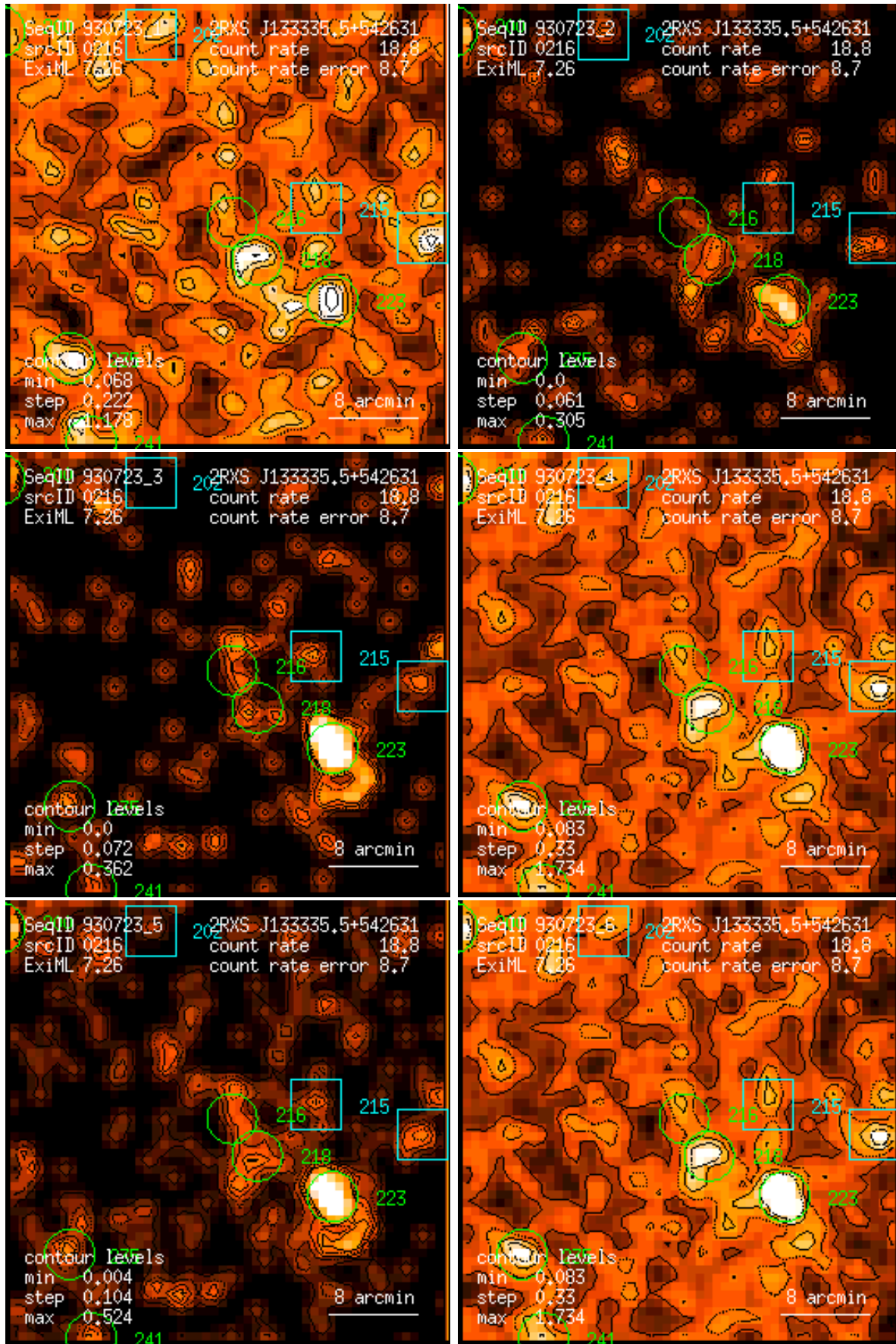
Figure 216: RASS 930723: detection 0216: band rate images, Gaussian filter: (1) PSPC channels 11 – 41, (2) 52 – 90, (3) 91 – 201, (4) 11 – 235, (5) 52 – 201, (6) 11 – 201. Broad band rates in counts/ks. Band rate contour levels in counts/ks/arcmin 2 .
